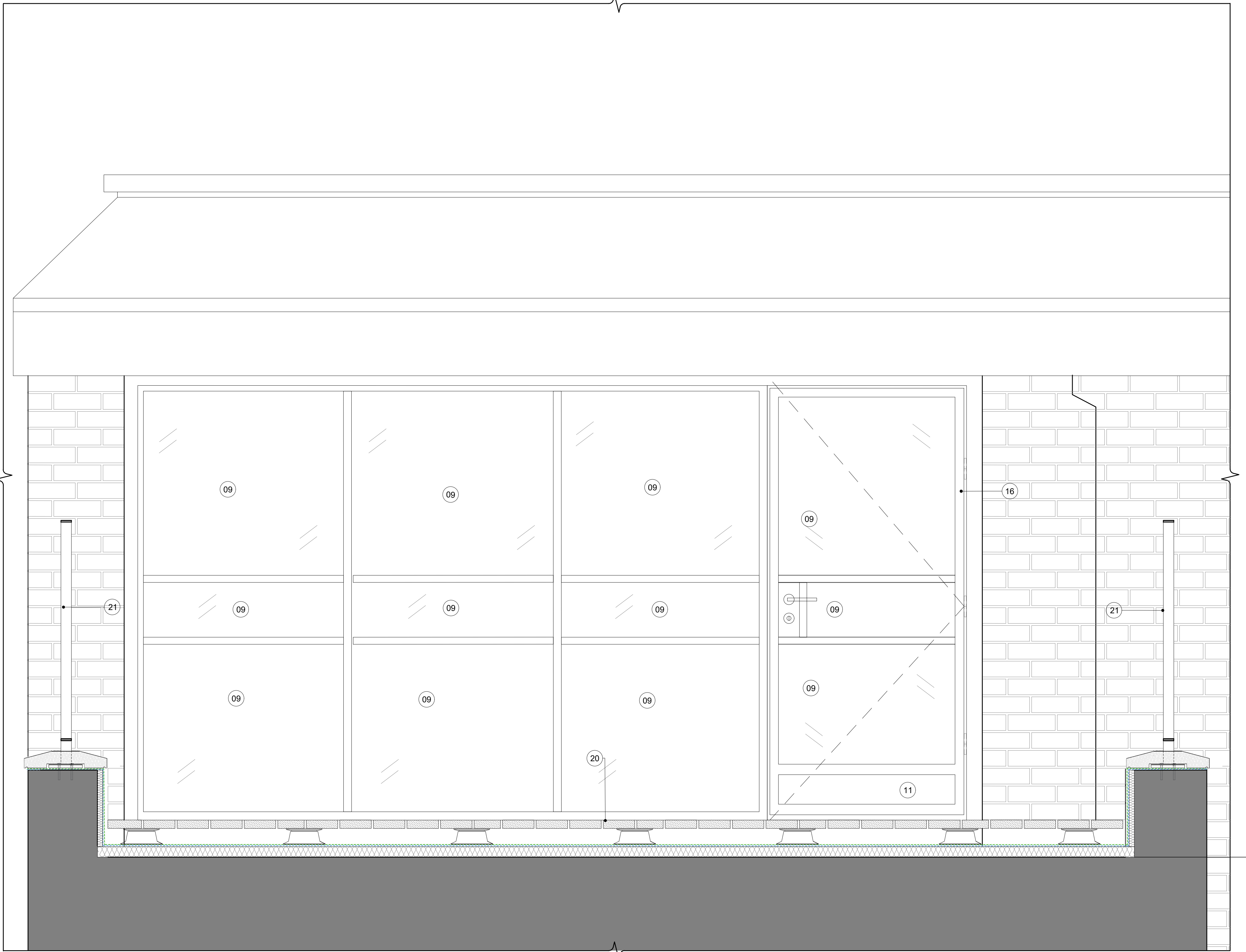
01 TYPICAL EXTERNAL TERRACE DOOR AND FIXED GLAZING A8150 ELEVATION
