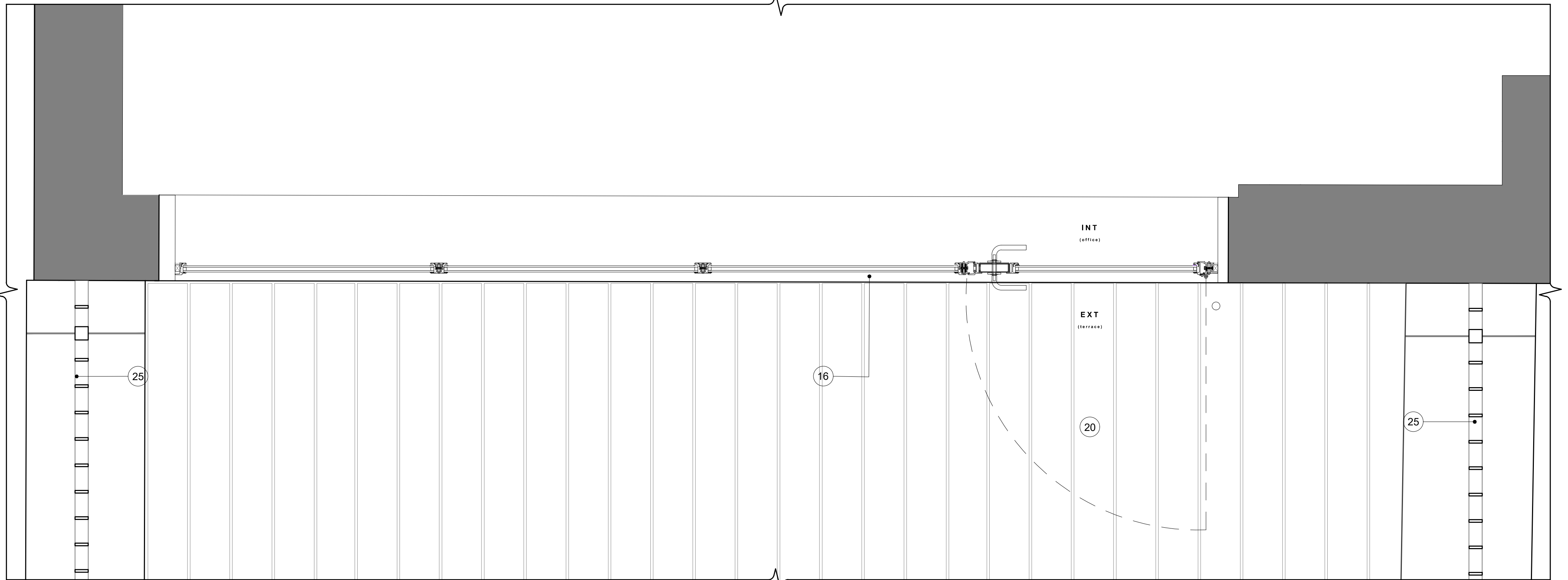
AA TYPICAL EXTERNAL TERRACE DOOR AND FIXED GLAZING A6150 PLAN
