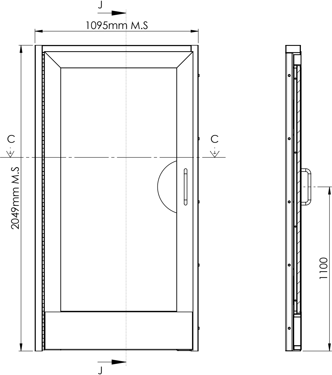
SECTION J-J
