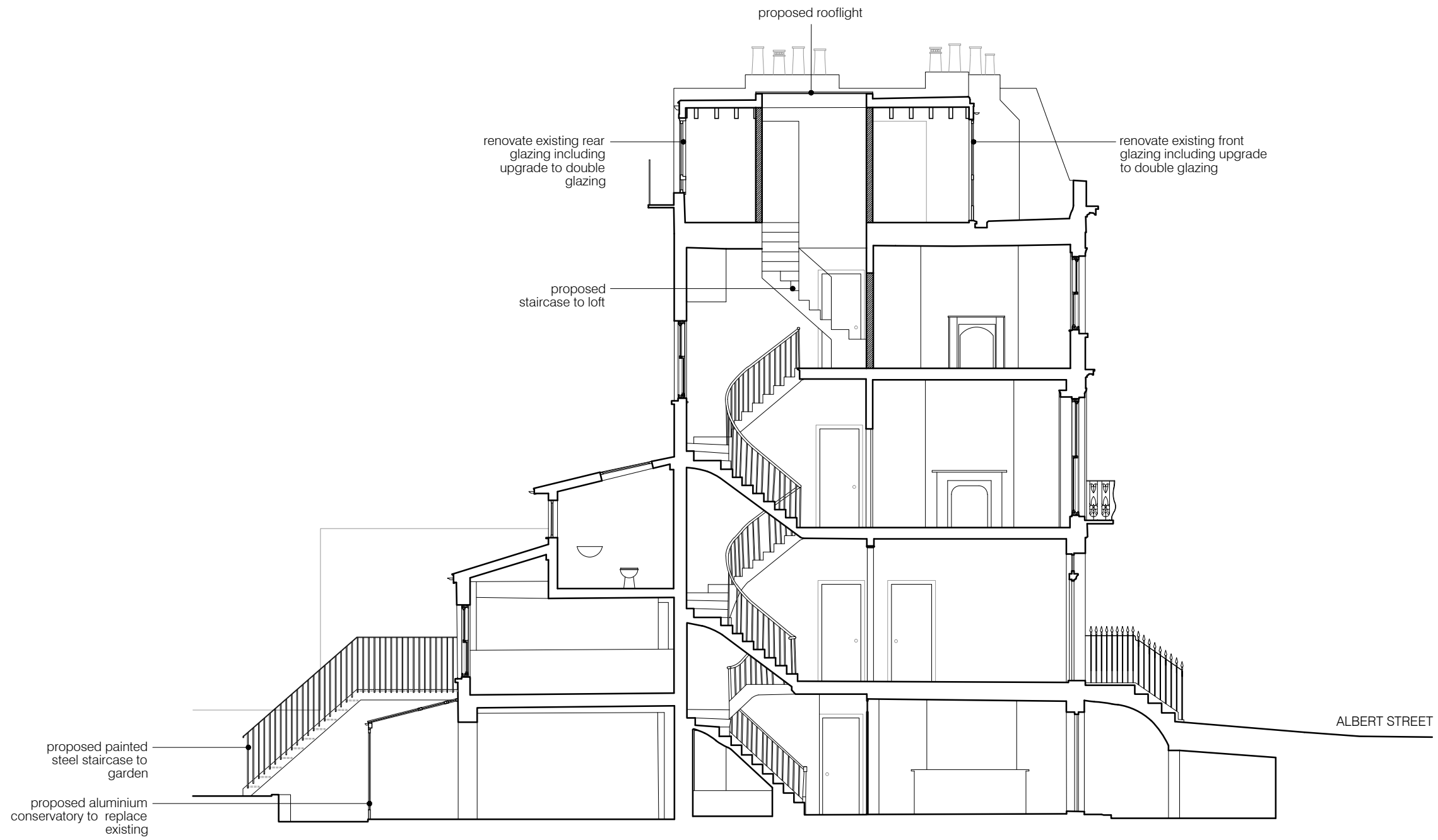
01 PROPOSED SECTION A-A scale 1:100
