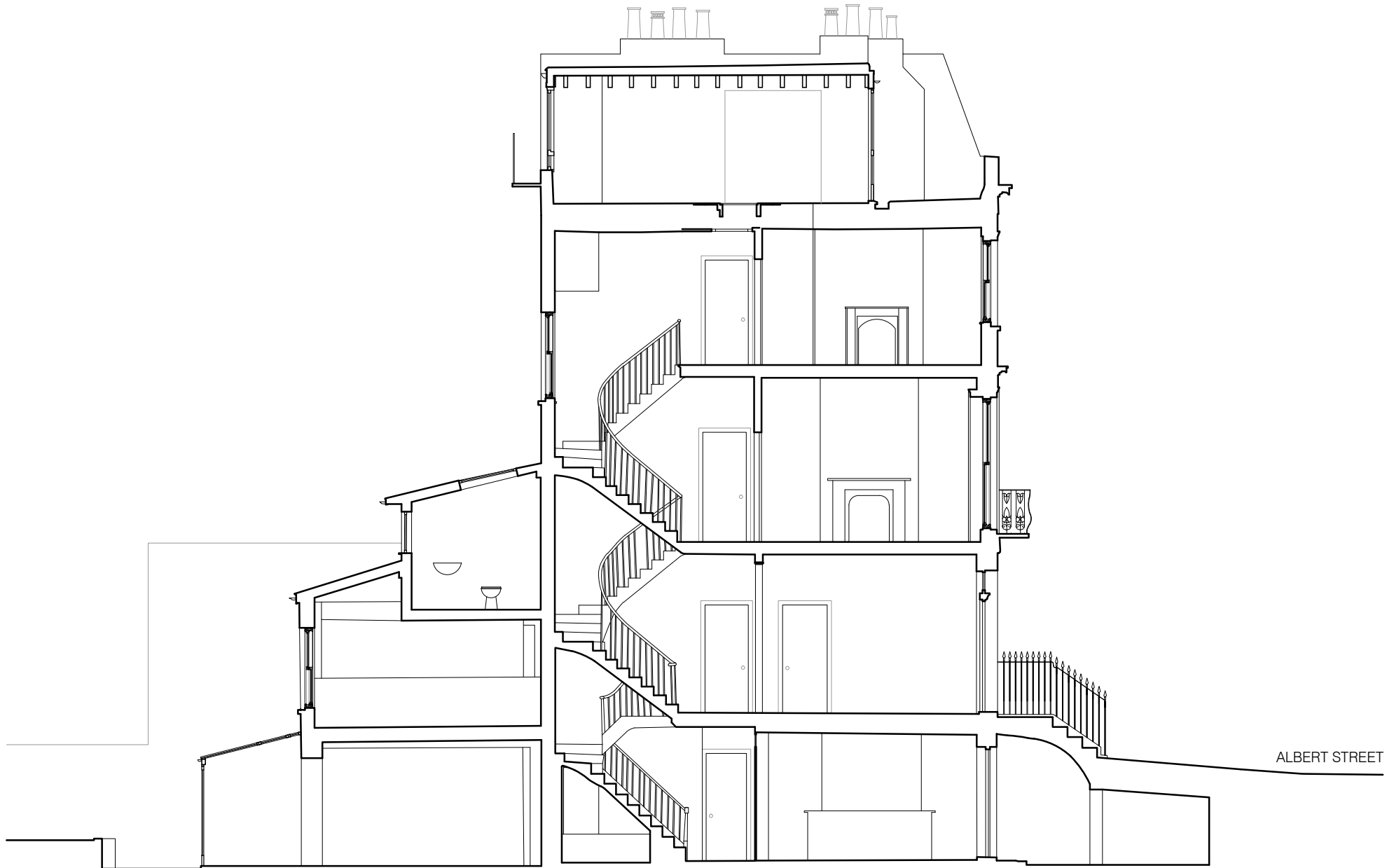
01 EXISTING SECTION A-A scale 1:100
