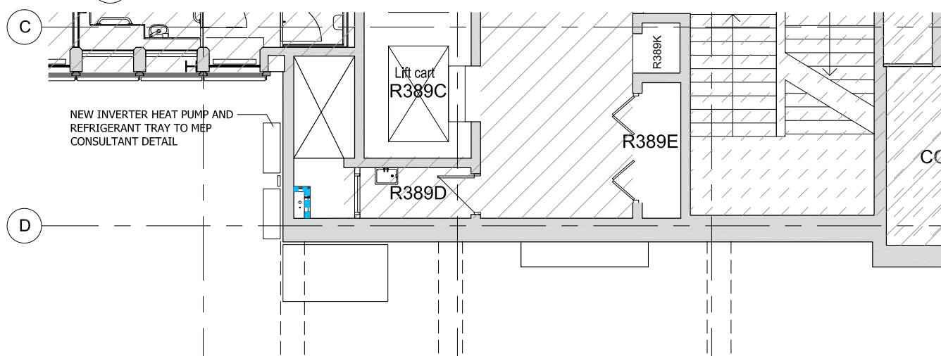
2 LEVEL 3 - CORE B PLAN - AS PROPOSED 1:50
