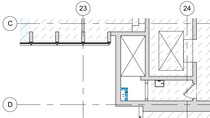
4 LEVELS 5-9 - CORE B PLAN - AS PROPOSED 1:50
