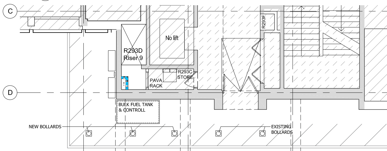
1 LEVEL 2 - CORE B PLAN - AS PROPOSED 1:50
