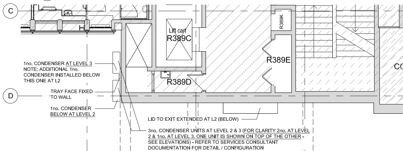
2 LEVEL 3 - CORE B PLAN - AS EXISTING 1:50
