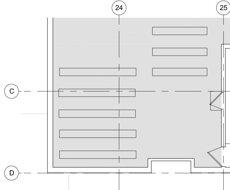
7 LEVEL 12 - CORE B PLAN - AS EXISTING 1:50
