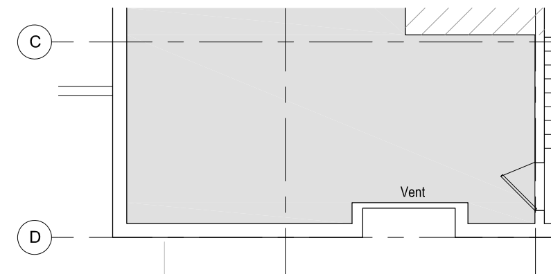
5 LEVELS 10-10.5 - CORE B PLAN - AS EXISTING 1:50
