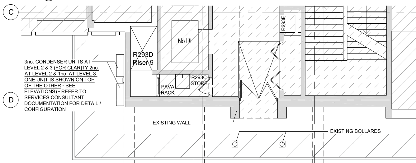
1 LEVEL 2 - CORE B PLAN - AS EXISTING 1:50
