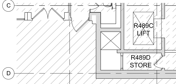
3 LEVEL 4 - CORE B PLAN - AS EXISTING 1:50
