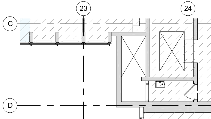
4 LEVELS 5-9 - CORE B PLAN - AS EXISTING 1:50
