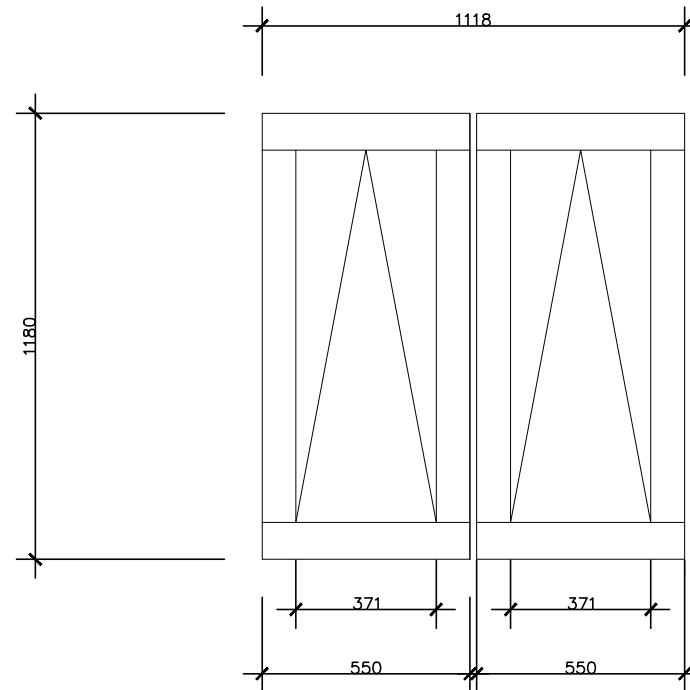
PROPOSED REAR VELUX WINDOW EXTERNAL MEASUREMENTS No. 6 PRIMROSE HILL STUDIOS
