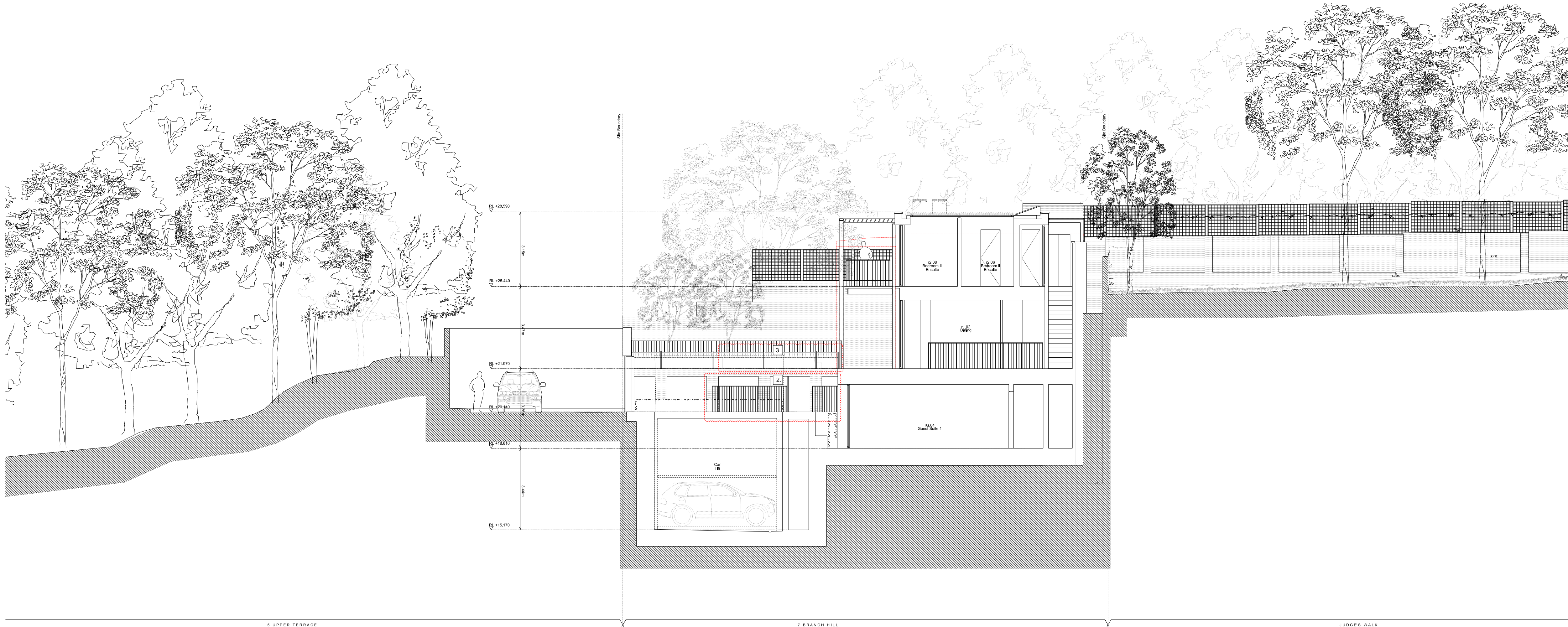
Proposed Section DD
