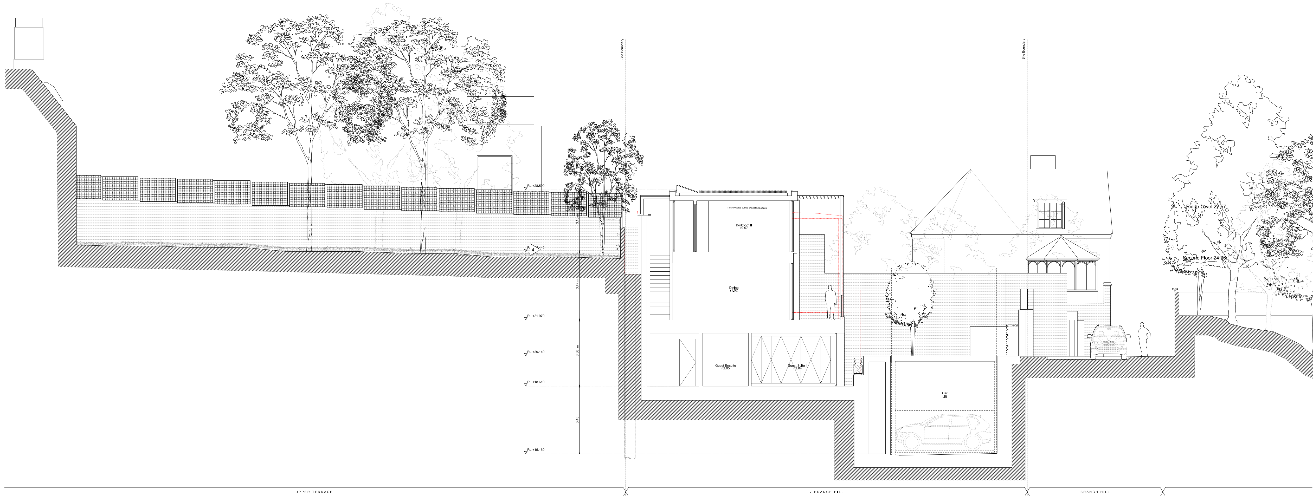
Existing Section CC
