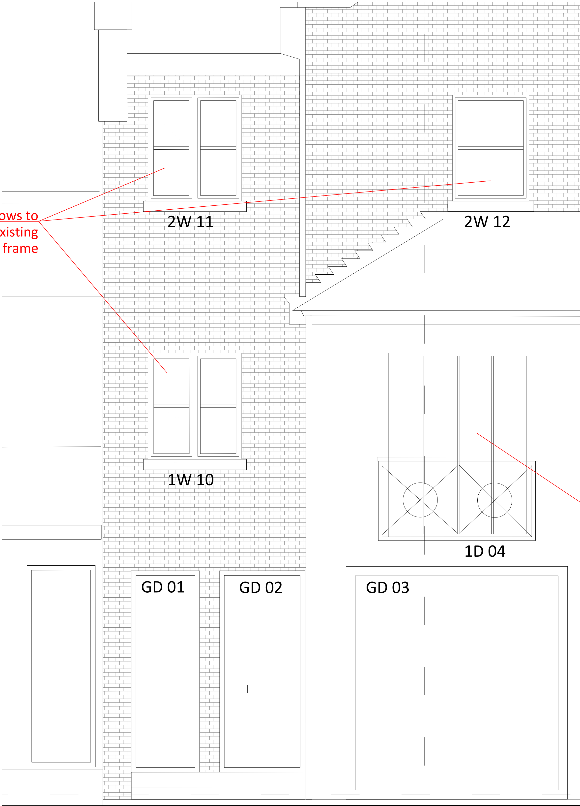
2 Proposed Detail Proposed Window and Door Detail 1:20
