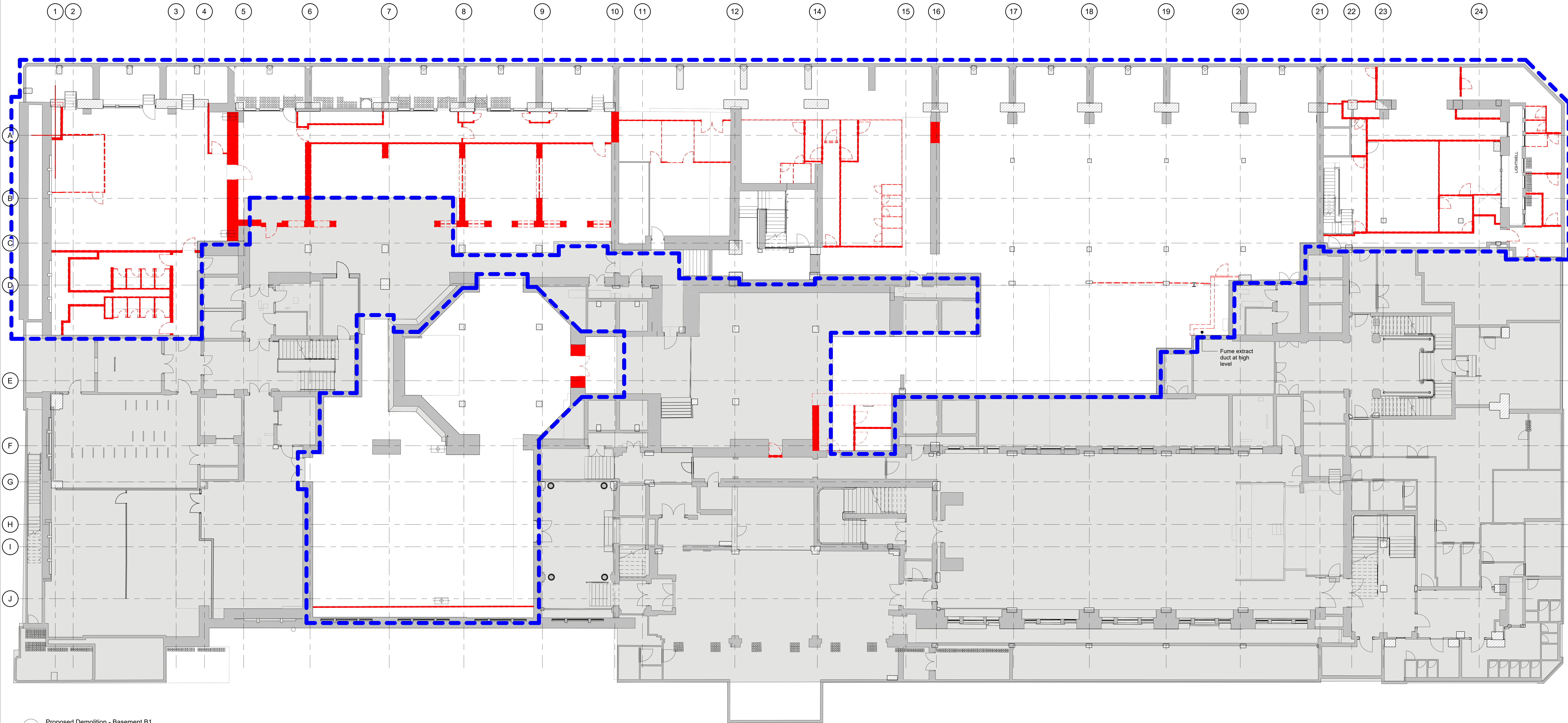
1 Proposed Demolition - Basement B1
