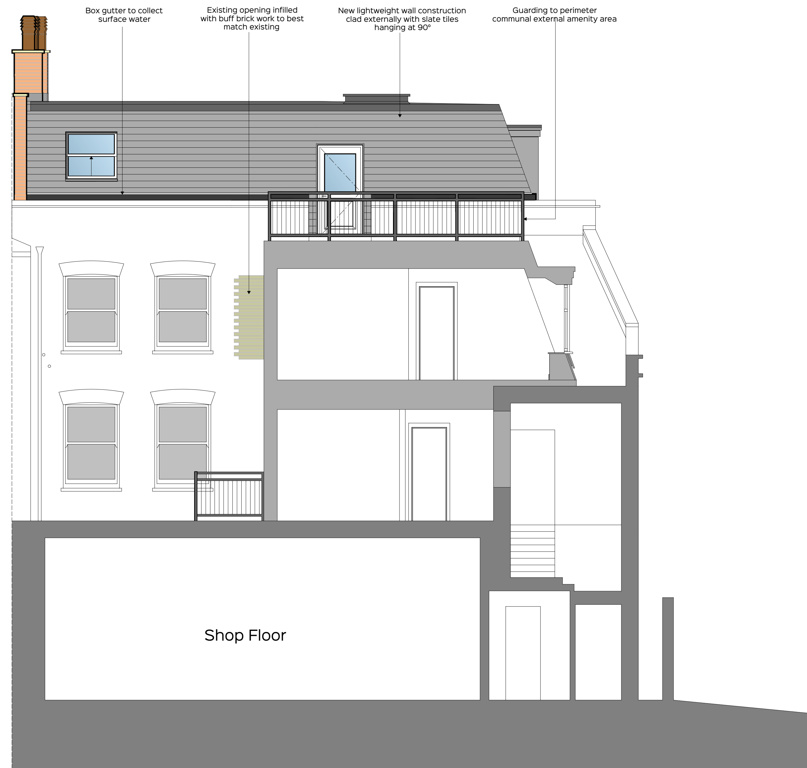
Proposed Section B-B (scale 1:50)
