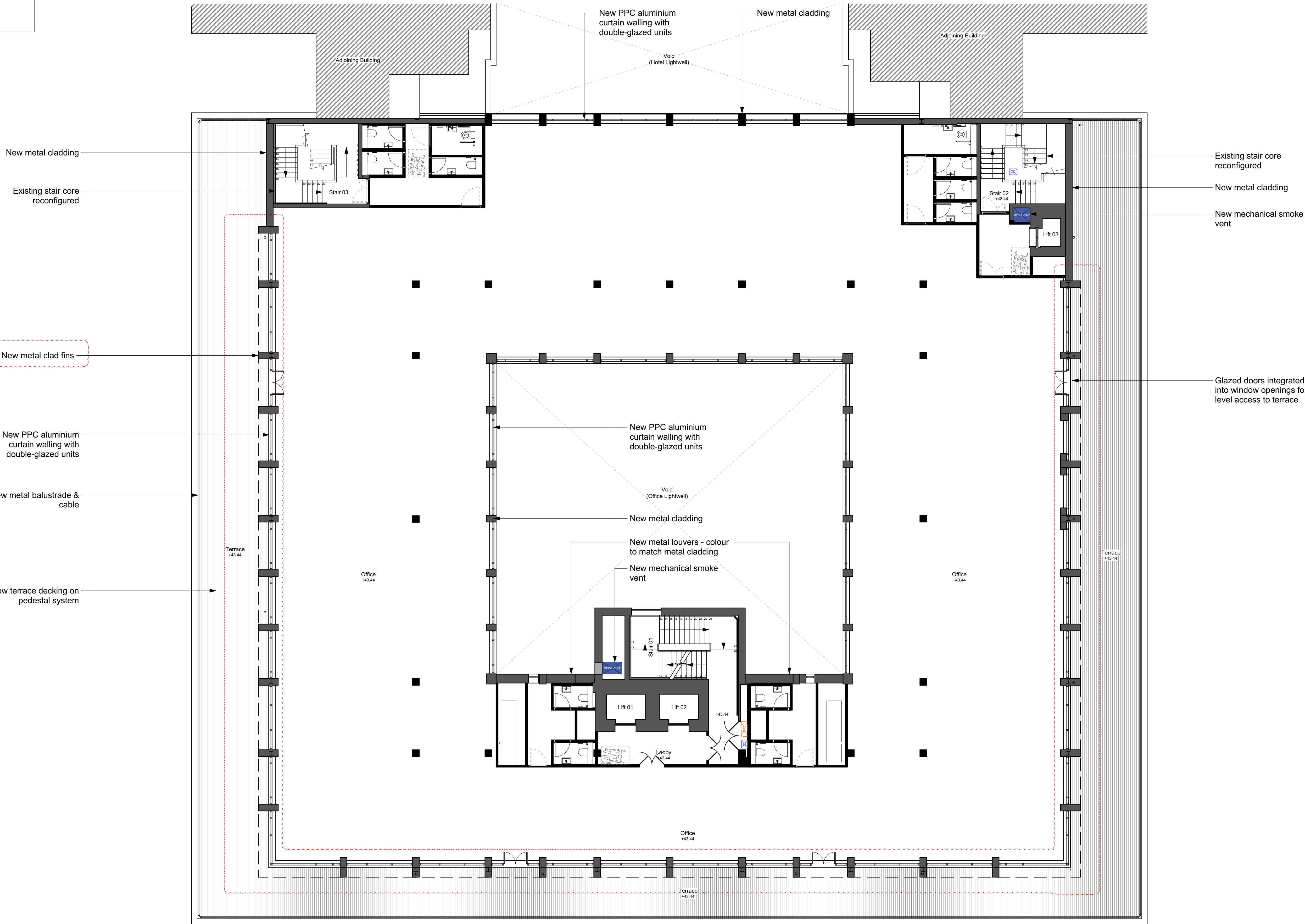
1 Proposed 5th Floor Plan Scale: 1:100
