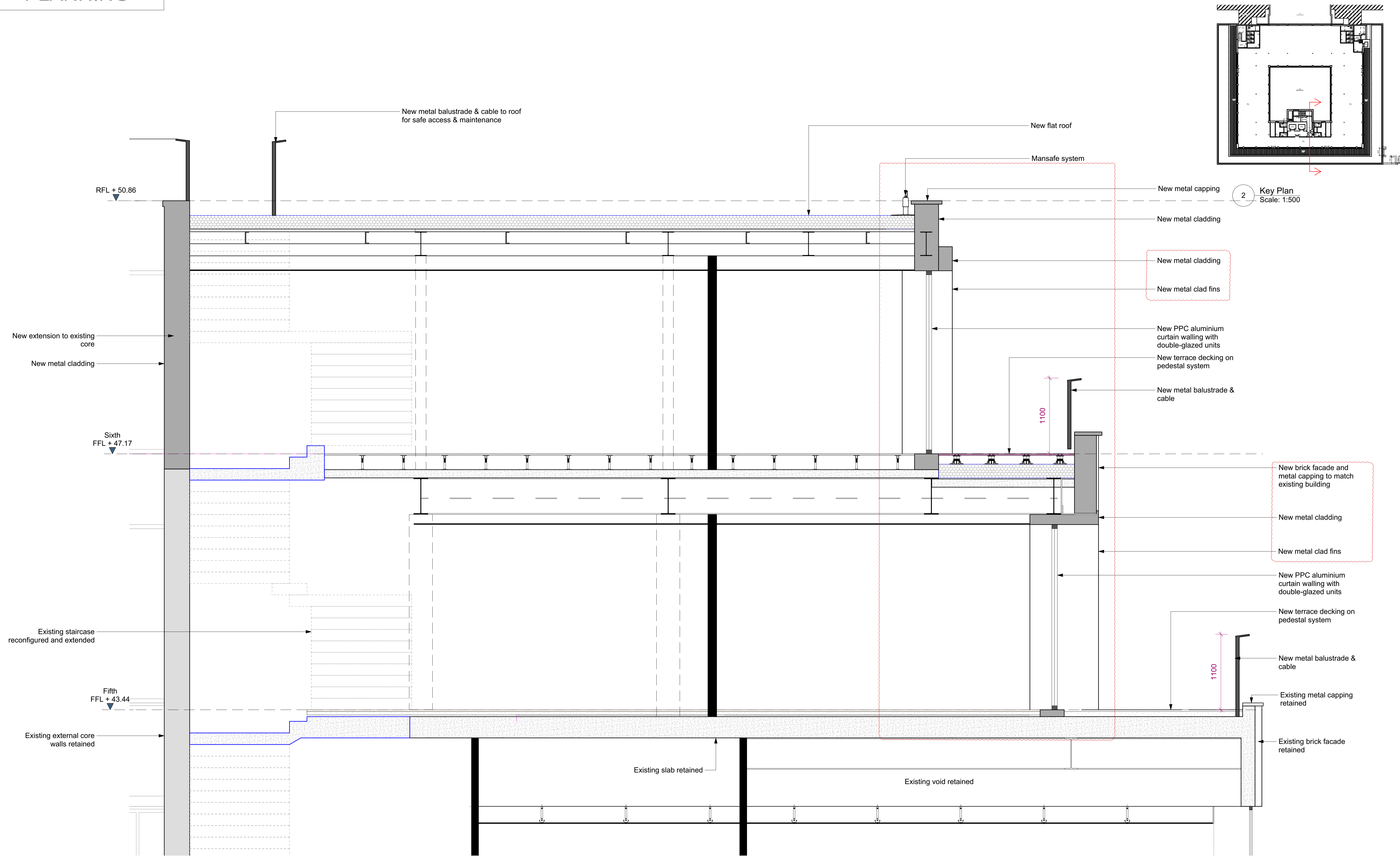
1 Proposed Detailed North-South Cross Section - 5th & 6th Floors Scale: 1:25
