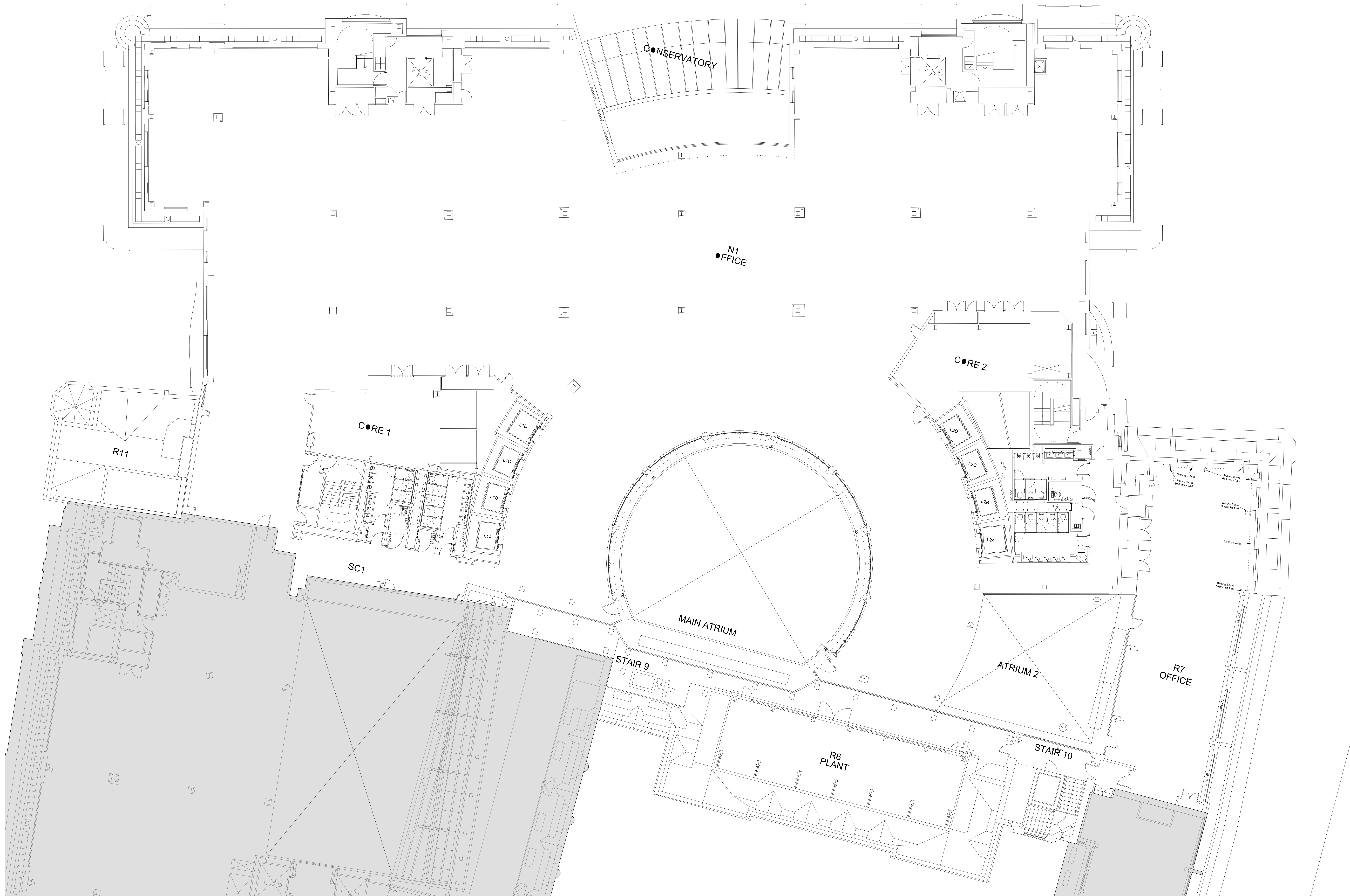
05 - Existing Fifth Floor Plan Scale: 1 : 100
