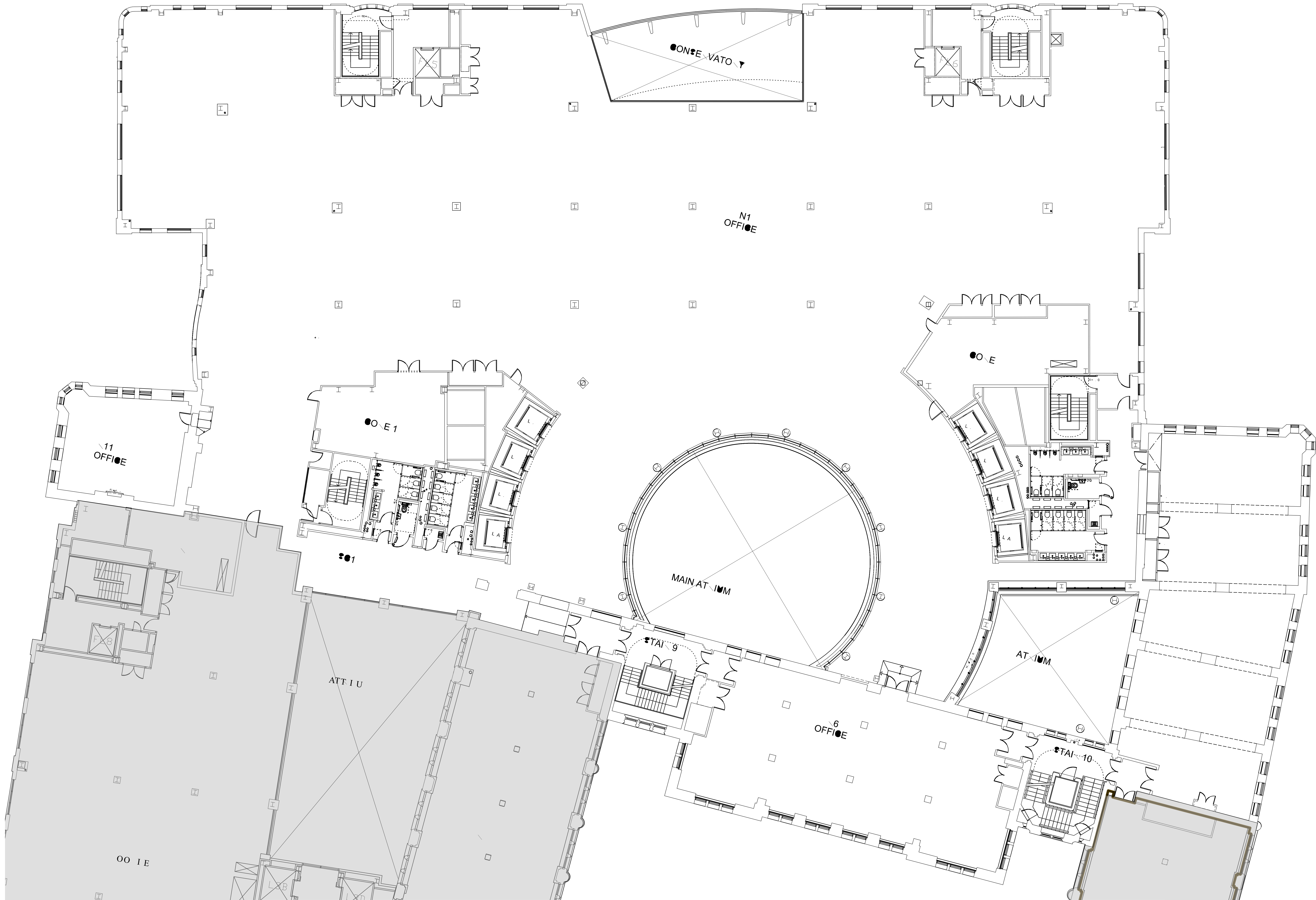
02 - Existing Second Floor Plan Scale: 1 : 100
