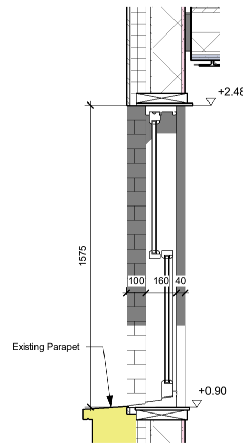
2 Win-01,02,03,05 DET_Section 1 : 20
