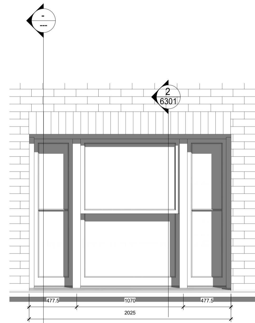
1 Win-01,02,03,05 DET_Elevation Section BB1
