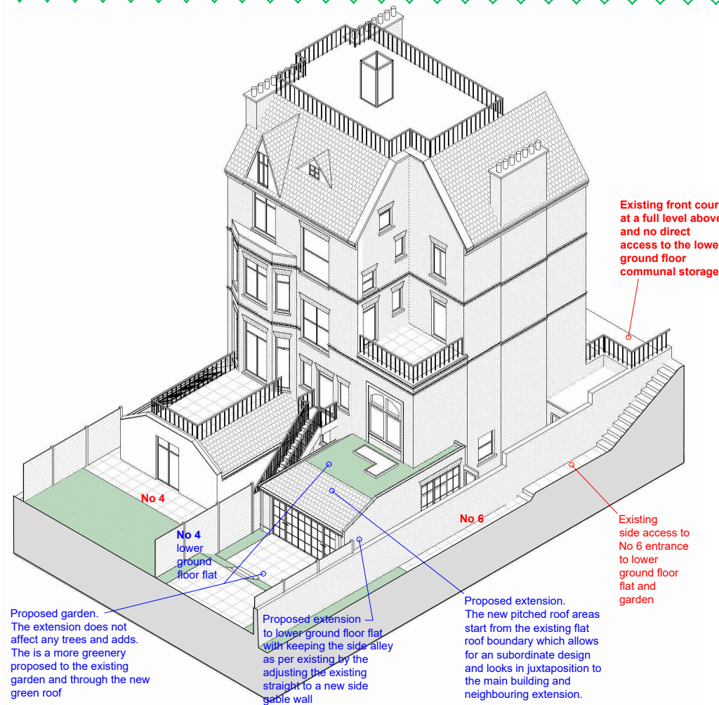
2 PROPOSED SOUTH WEST ISOMETRIC PREVIEW (REAR OF NO 6 & NO 4 STRATHRAY GARDENS)
