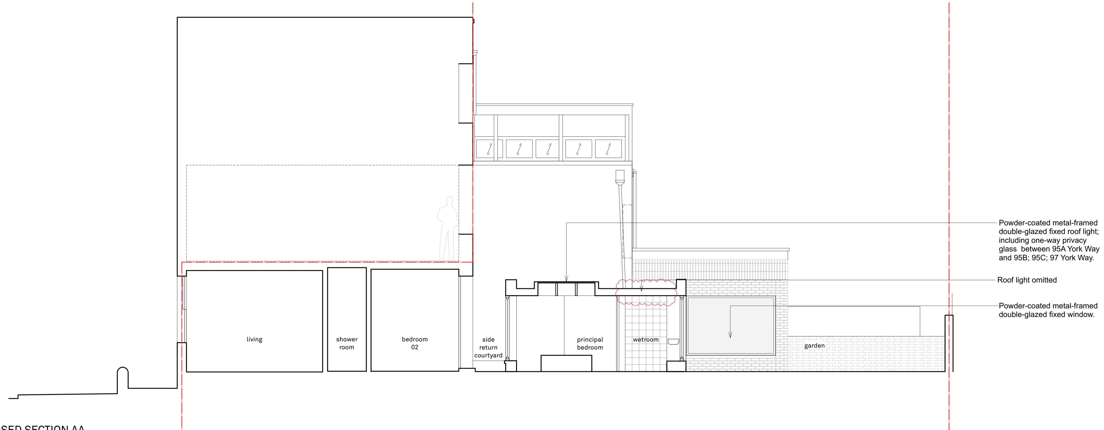
1 PROPOSED SECTION AA Scale: 1:50 @ A1 / 1:100 @ A3
