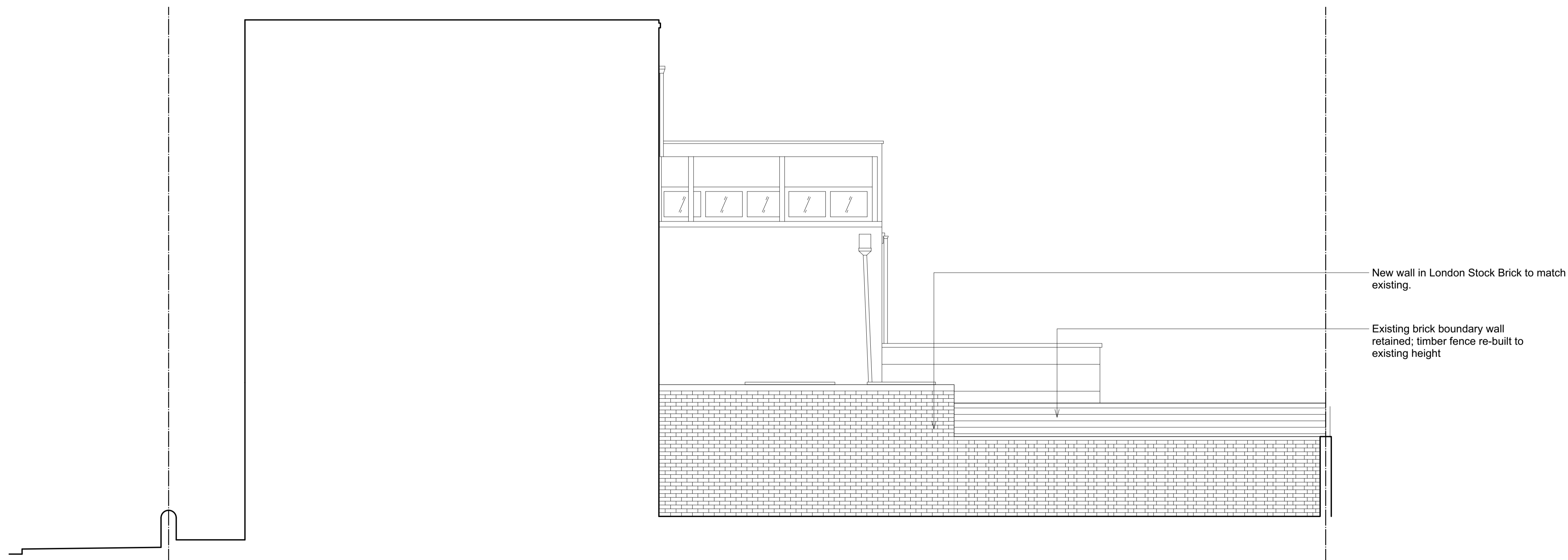
2 PROPOSED SIDE ELEVATION (FROM No.97 YORK WAY) Scale: 1:50 @ A1 / 1:100 @ A3
