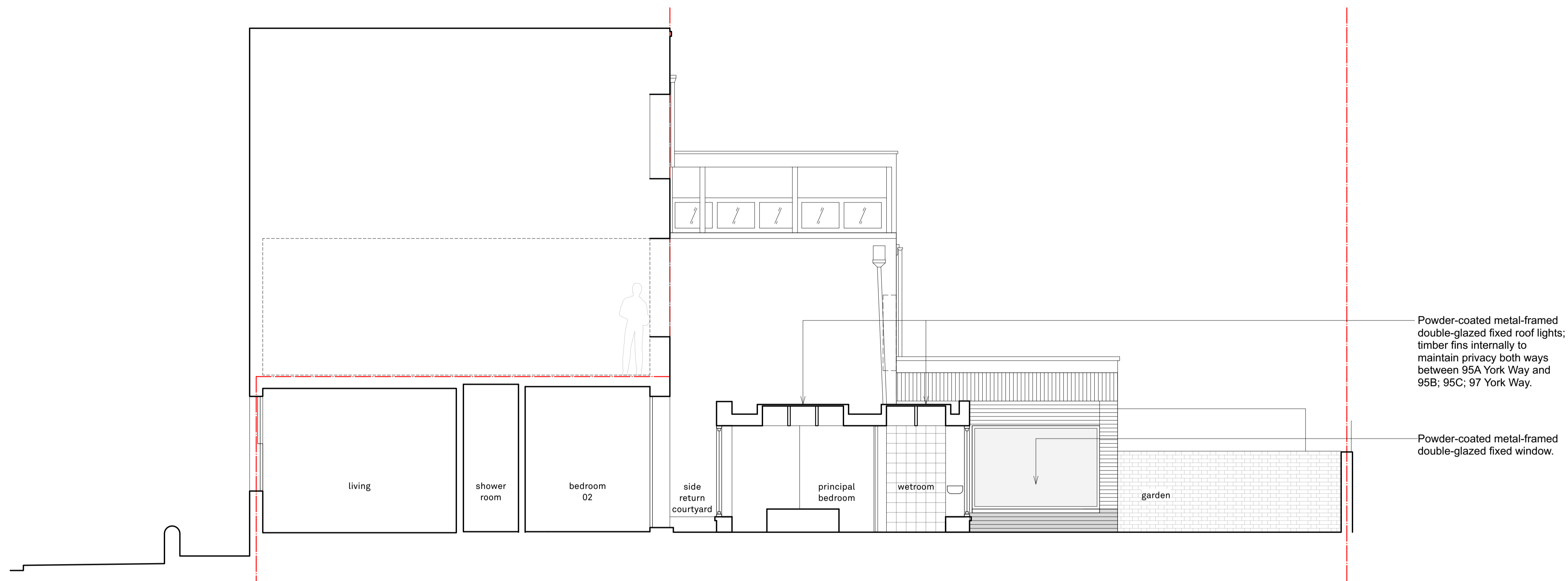
1 PROPOSED SECTION AA Scale: 1:50 @ A1 / 1:100 @ A3
