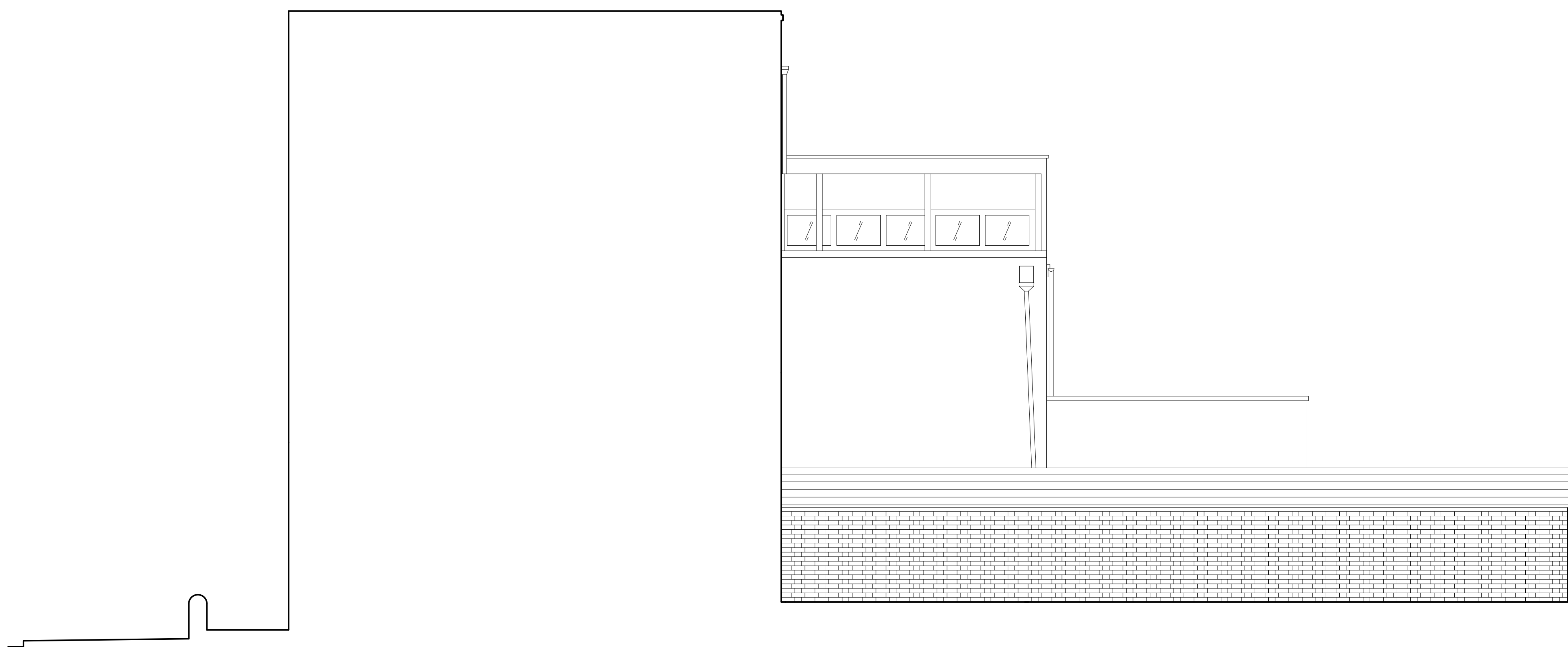
2 EXISTING SIDE ELEVATION (FROM No.97 YORK WAY) Scale: 1:50 @ A1 / 1:100 @ A3
