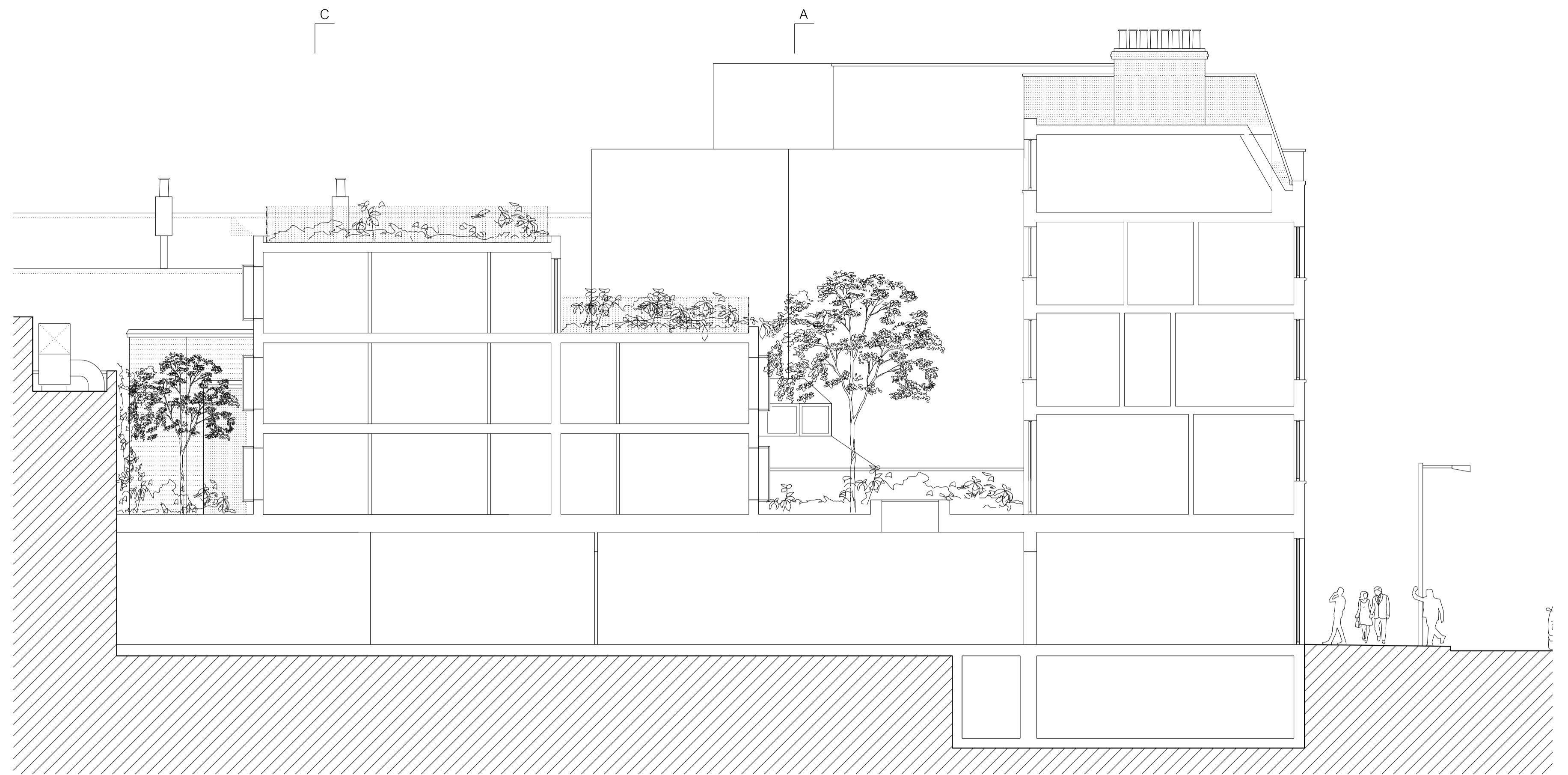
② SECTION B
