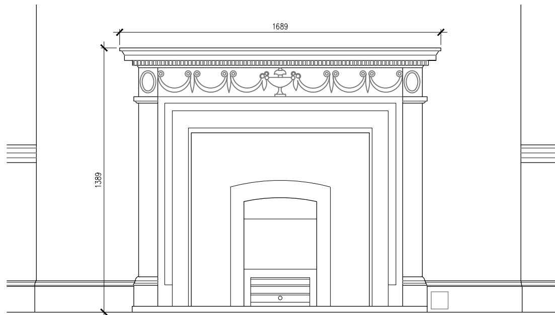
EXISTING FIRST FLOOR FIREPLACE - SCALE 1:20 @ A3 SITTING ROOM FIREPLACE
