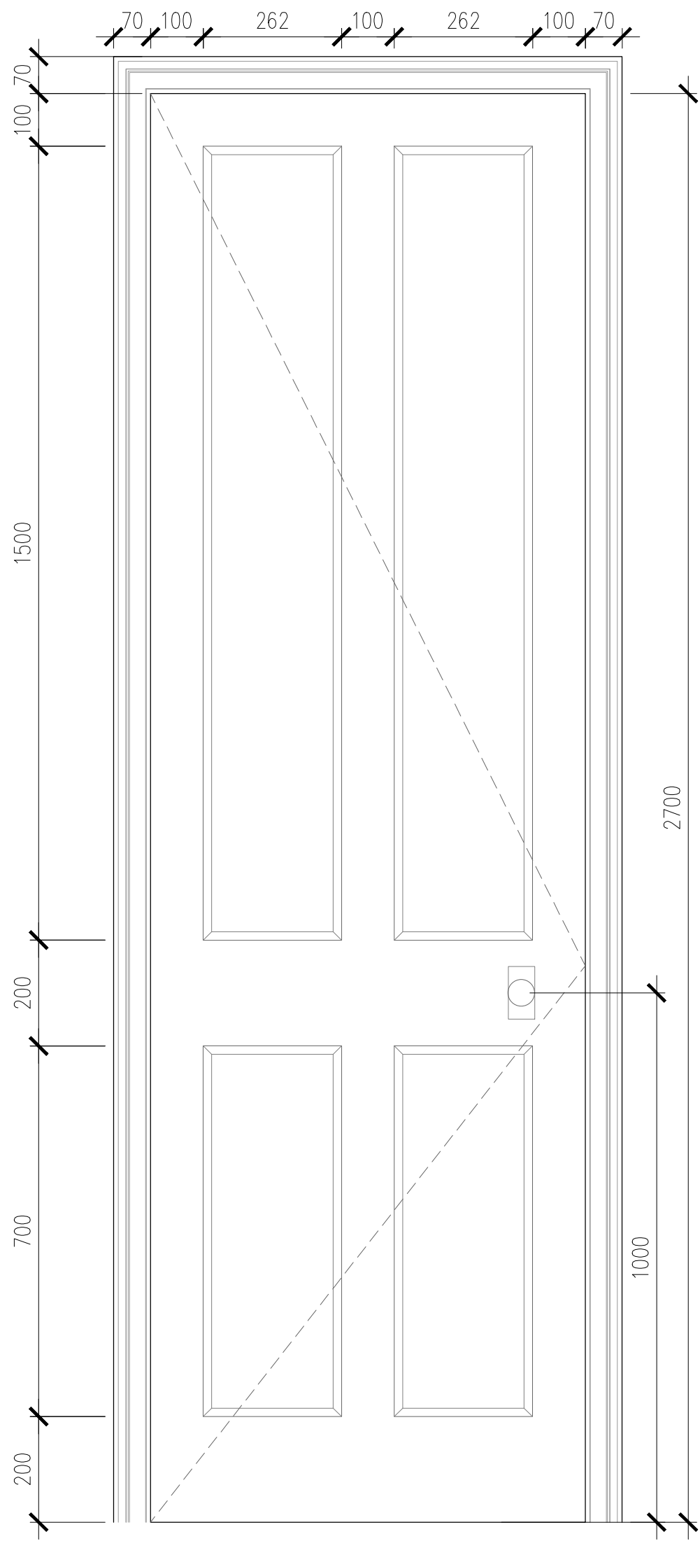
TYPICAL DOOR DETAIL 03 (FD30) HIERARCHY 3 REGENCY PERIOD, FOUR PANEL DOOR SCALE - 1:10
