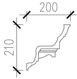
01 PROPOSED CORNICE PROFILE - COV1
