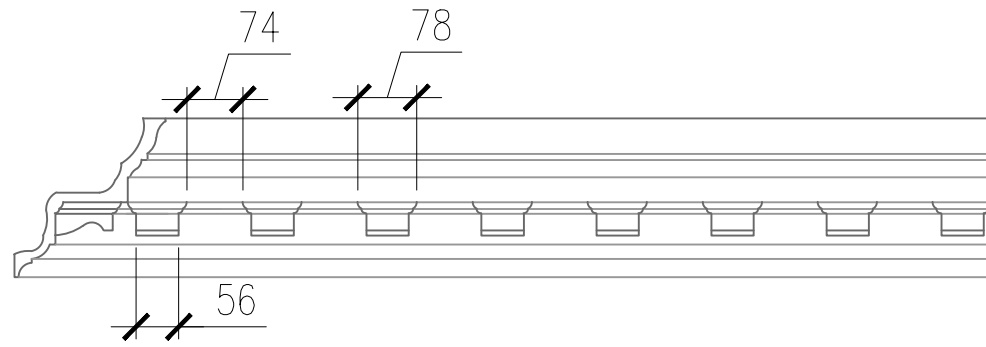
01 PROPOSED CORNICE ELEVATION - COV1 GROUND FLOOR ENTRANCE LOBBY FIRST FLOOR STAIR LANDING
