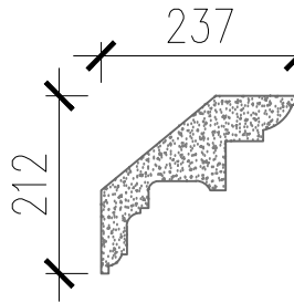
03 PROPOSED CORNICE PROFILE - COV3
