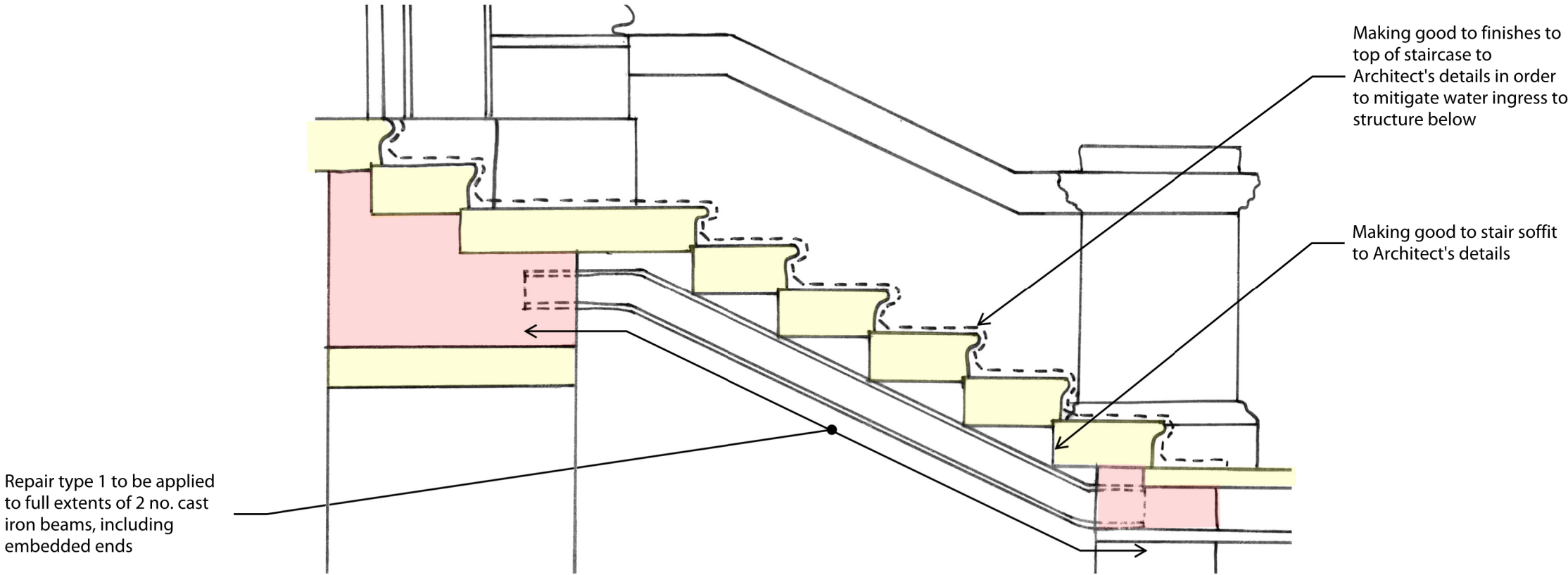
SECTION 1-1 (1:20)
