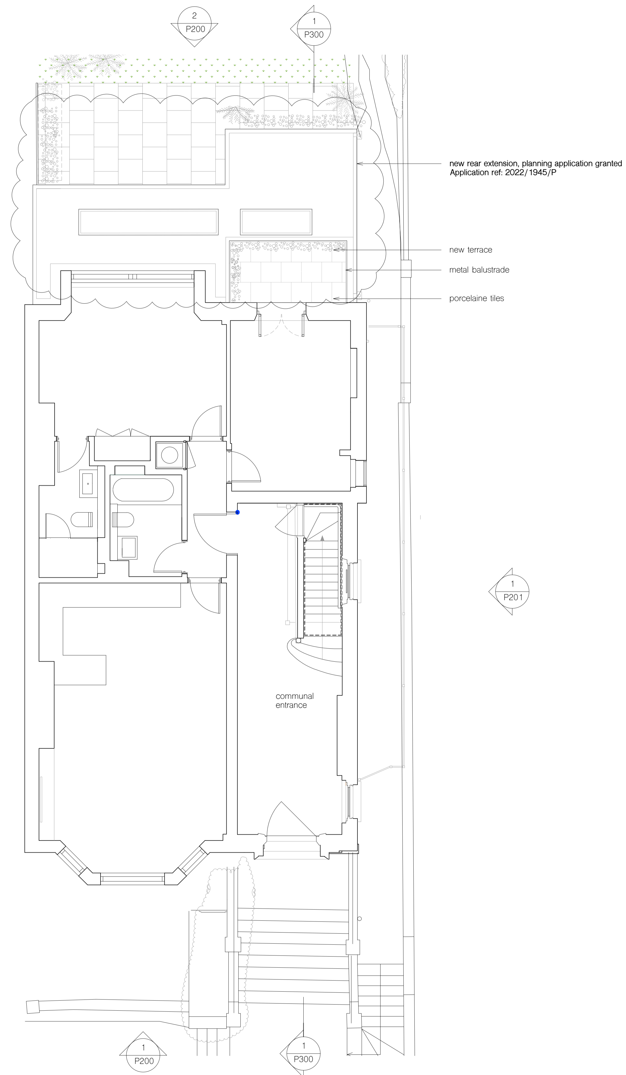
1 ground floor / roof plan
