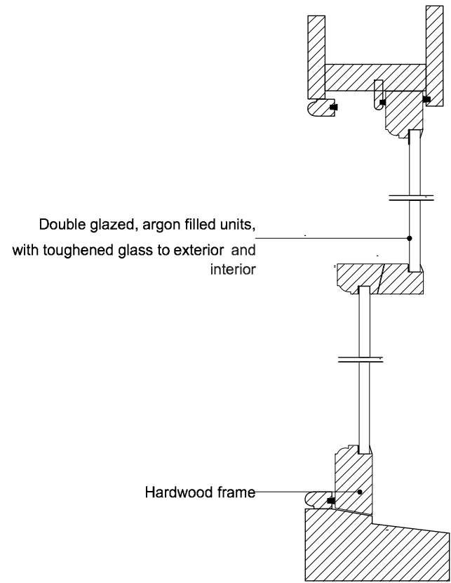
TYPICAL SASH WINDOW SECTION SCALE 1:5 @A3
