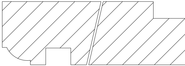
TYPICAL SASH WINDOW MEETING RAIL SCALE 1:1 @A3
