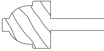
TYPICAL SASH WINDOW GLAZING BAR SCALE 1:1 @A3
