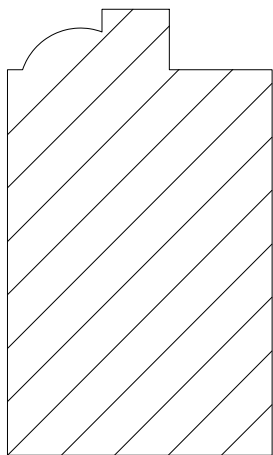
TYPICAL SASH WINDOW BOTTOM RAIL SCALE 1:1 @A3
