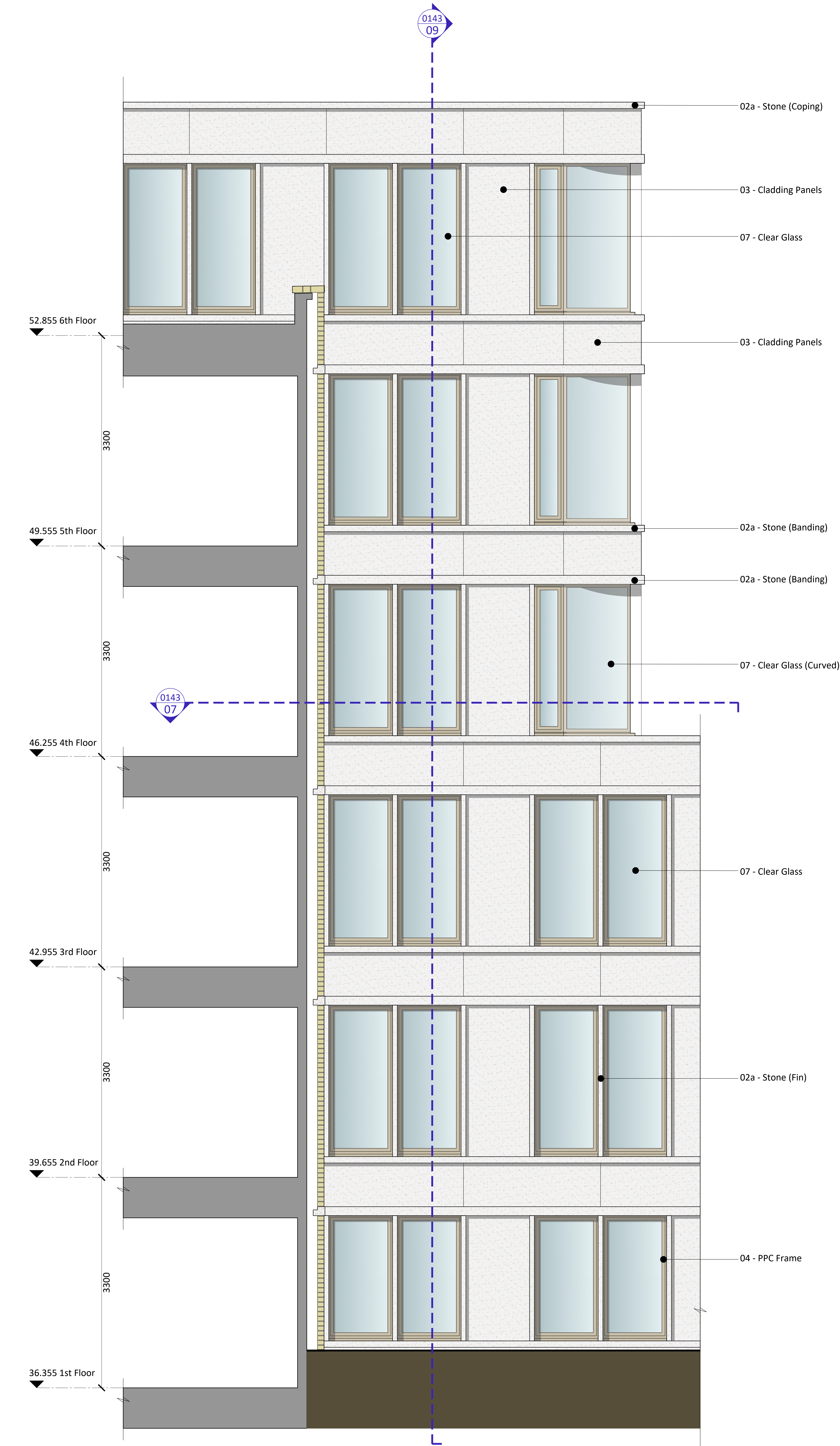
08 - Elevation - East (Int. Courtyard)
