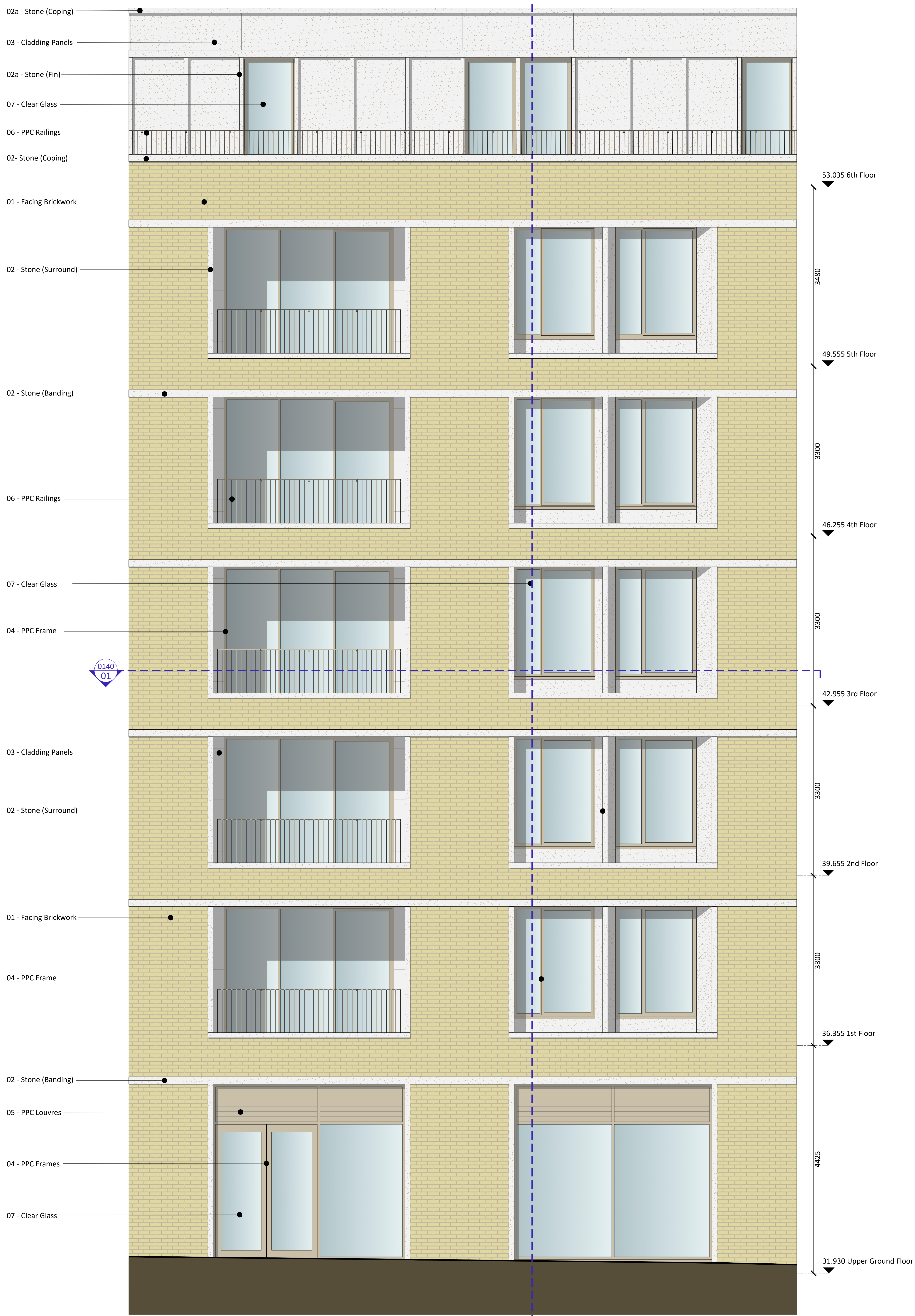
02 - Elevation - South (AR)
