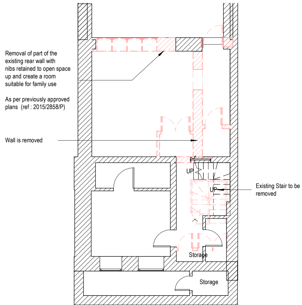
2 Demolish Lower Ground Floor Plan 1 : 100
