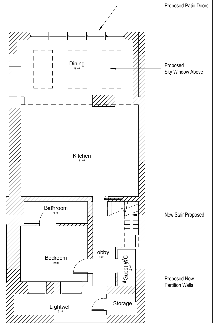
3 Proposed Lower Ground Floor Plan 1 : 100
