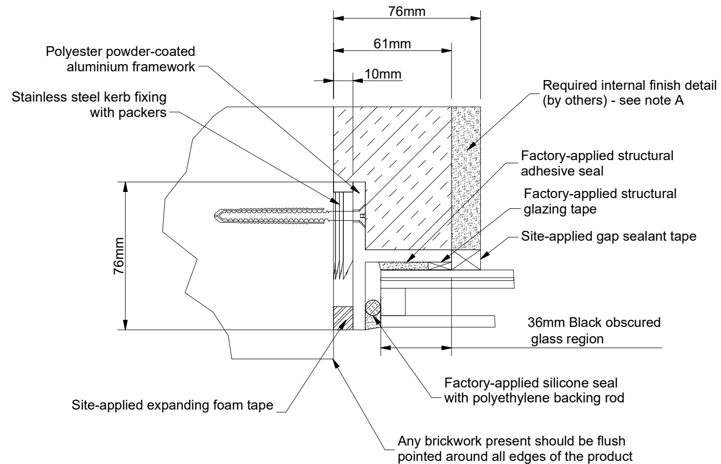
Detail E ( Scale 1 : 2 )
