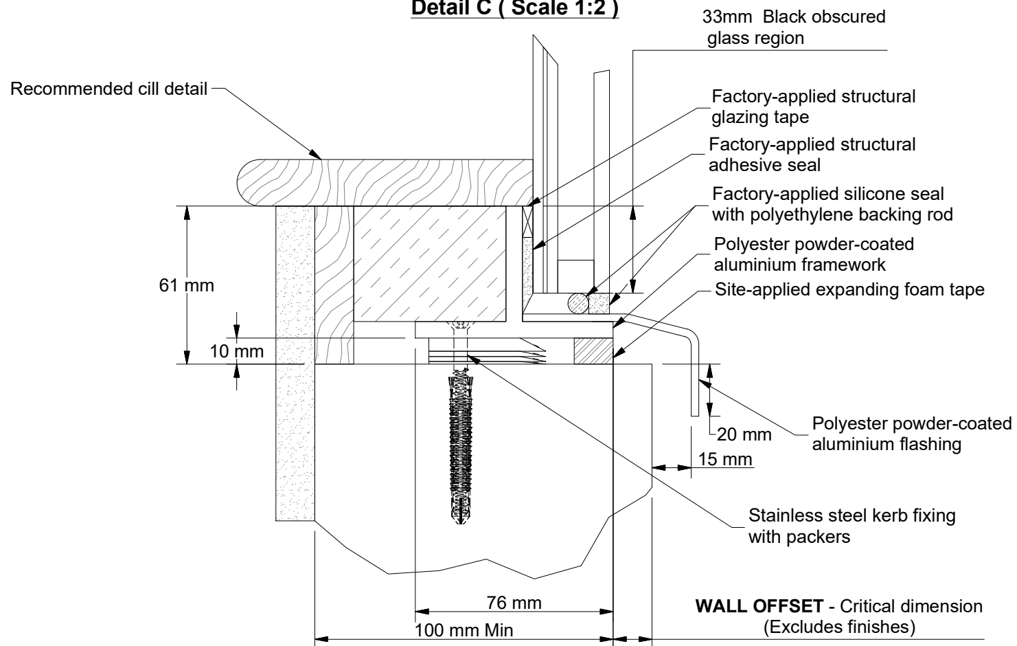
Detail C ( Scale 1:2 )
