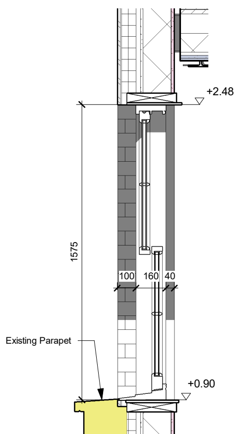
2 Win-01,02,03,05 DET_Section 1 : 20
