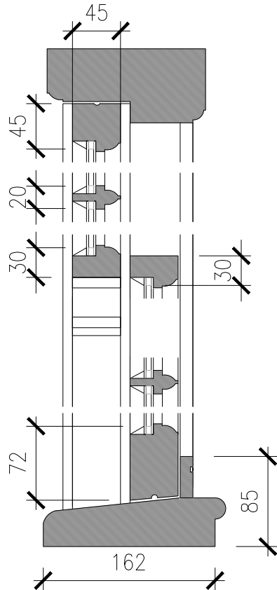
06 | PROPOSED TIMBER SASH WINDOW SECTION 1:5
