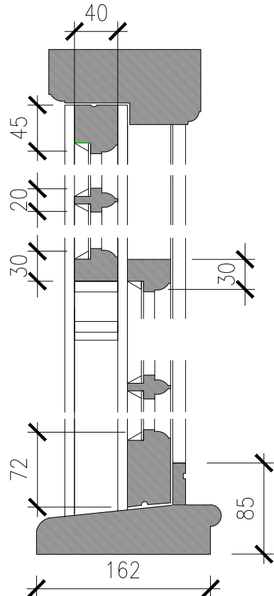
02 | EXISTING TIMBER SASH WINDOW SECTION 1:5
