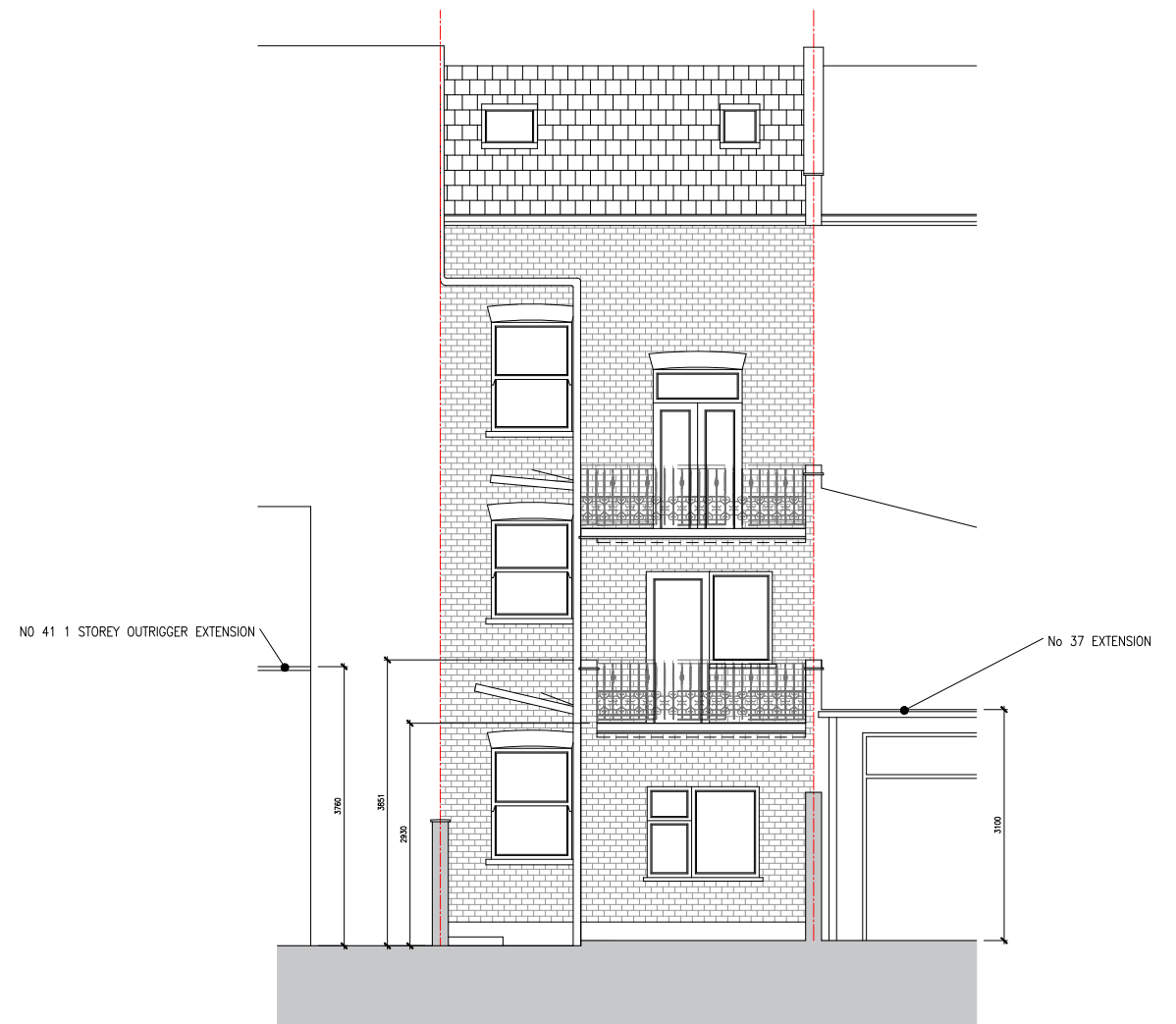
02 | EXISTING REAR ELEVATION
