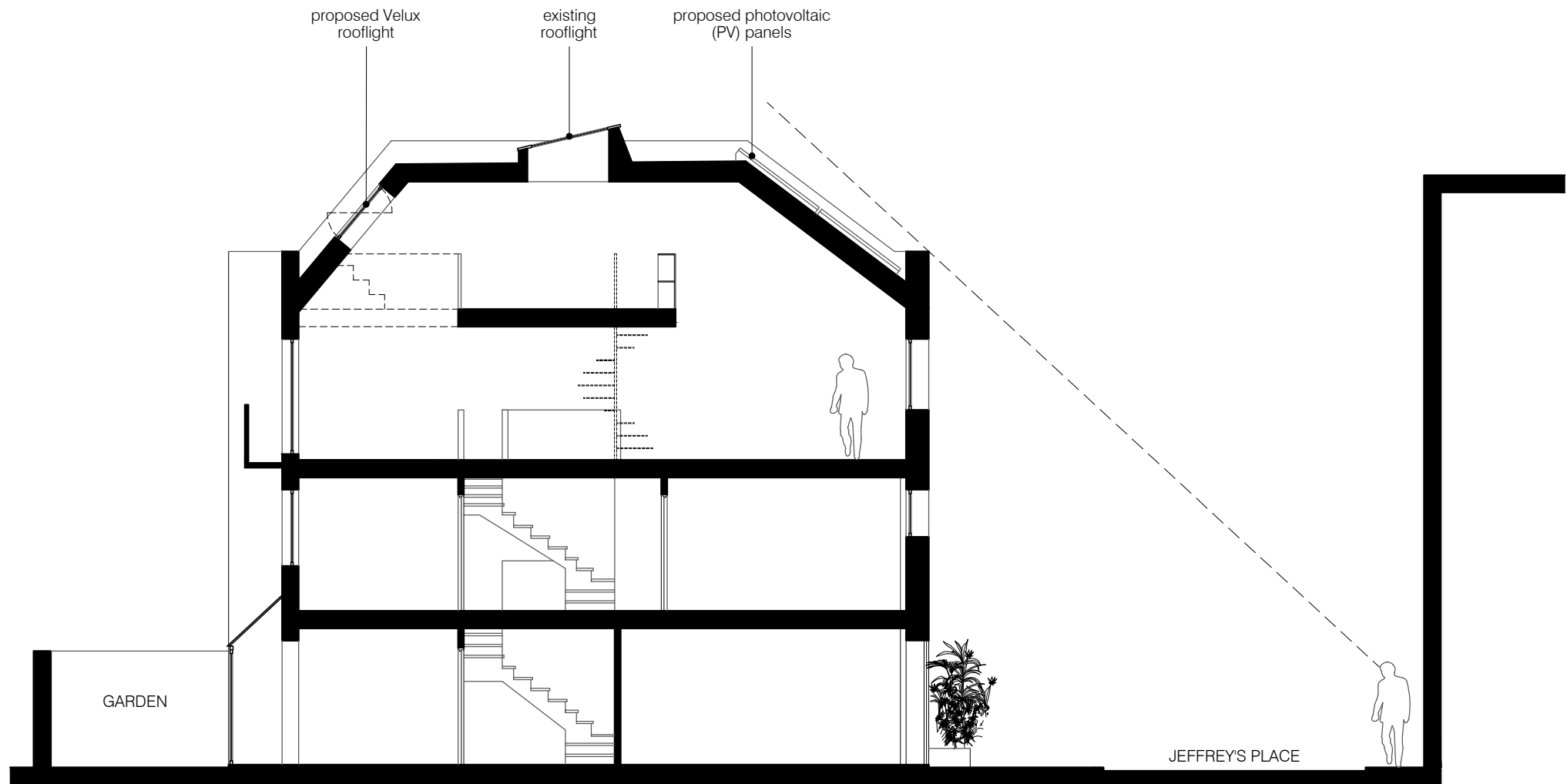
01 PROPOSED EXTENDED SECTION A-A scale 1:100
