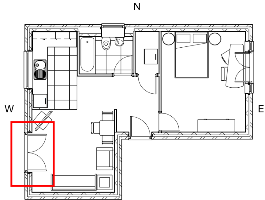
PROPOSED FLOORPLAN 1:100 @ A3
