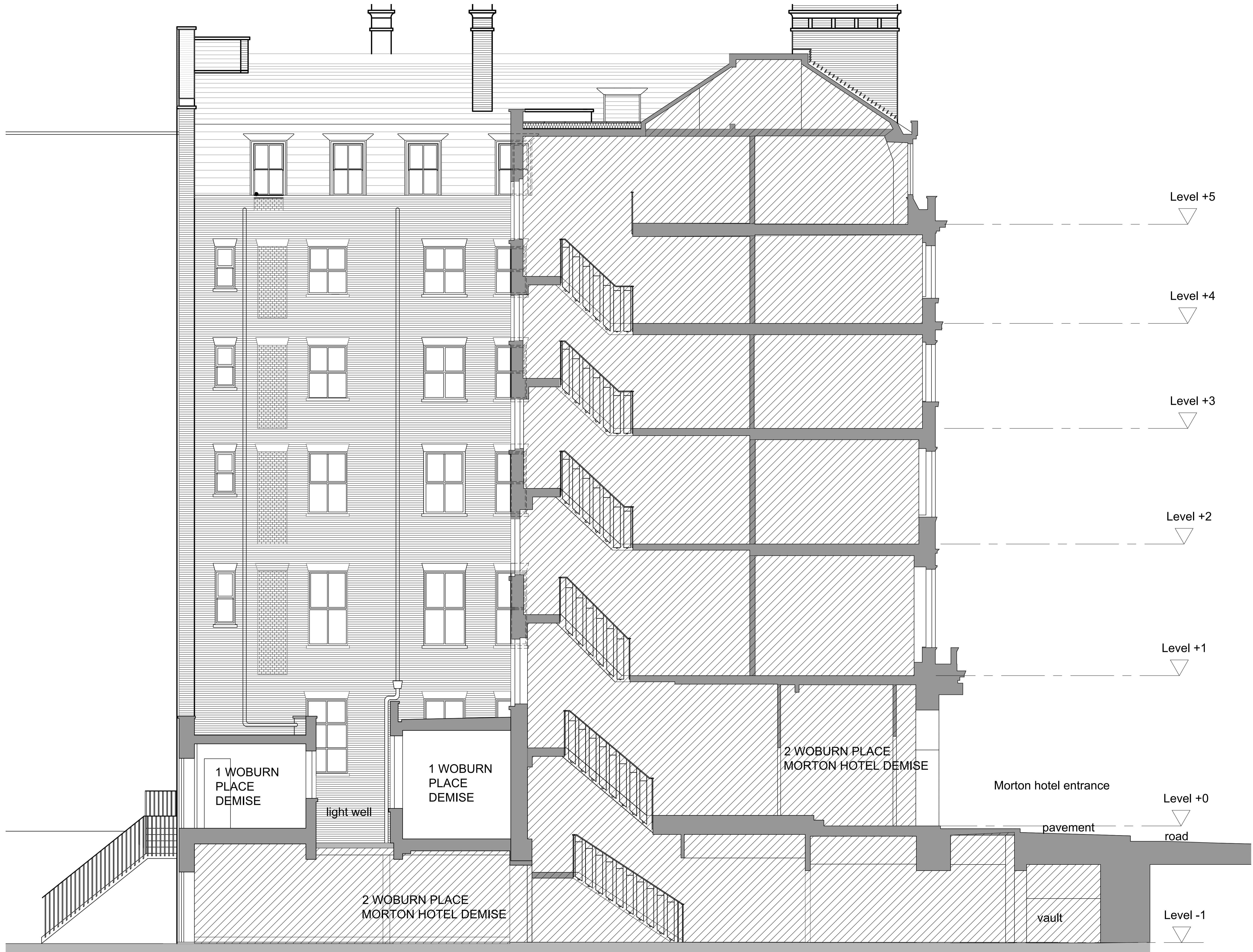
1 SECTION - AA -
