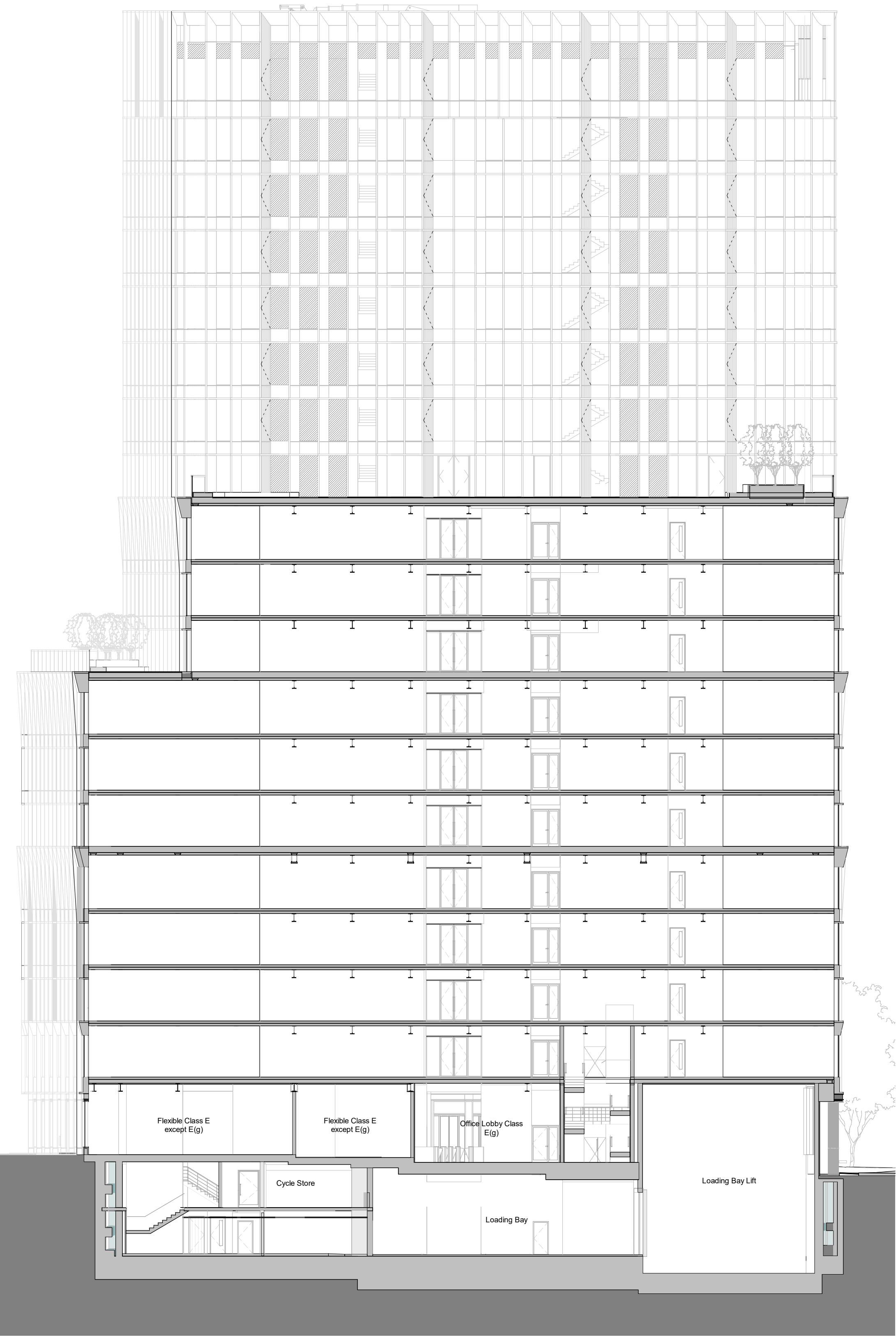
1MS Proposed Section DD
