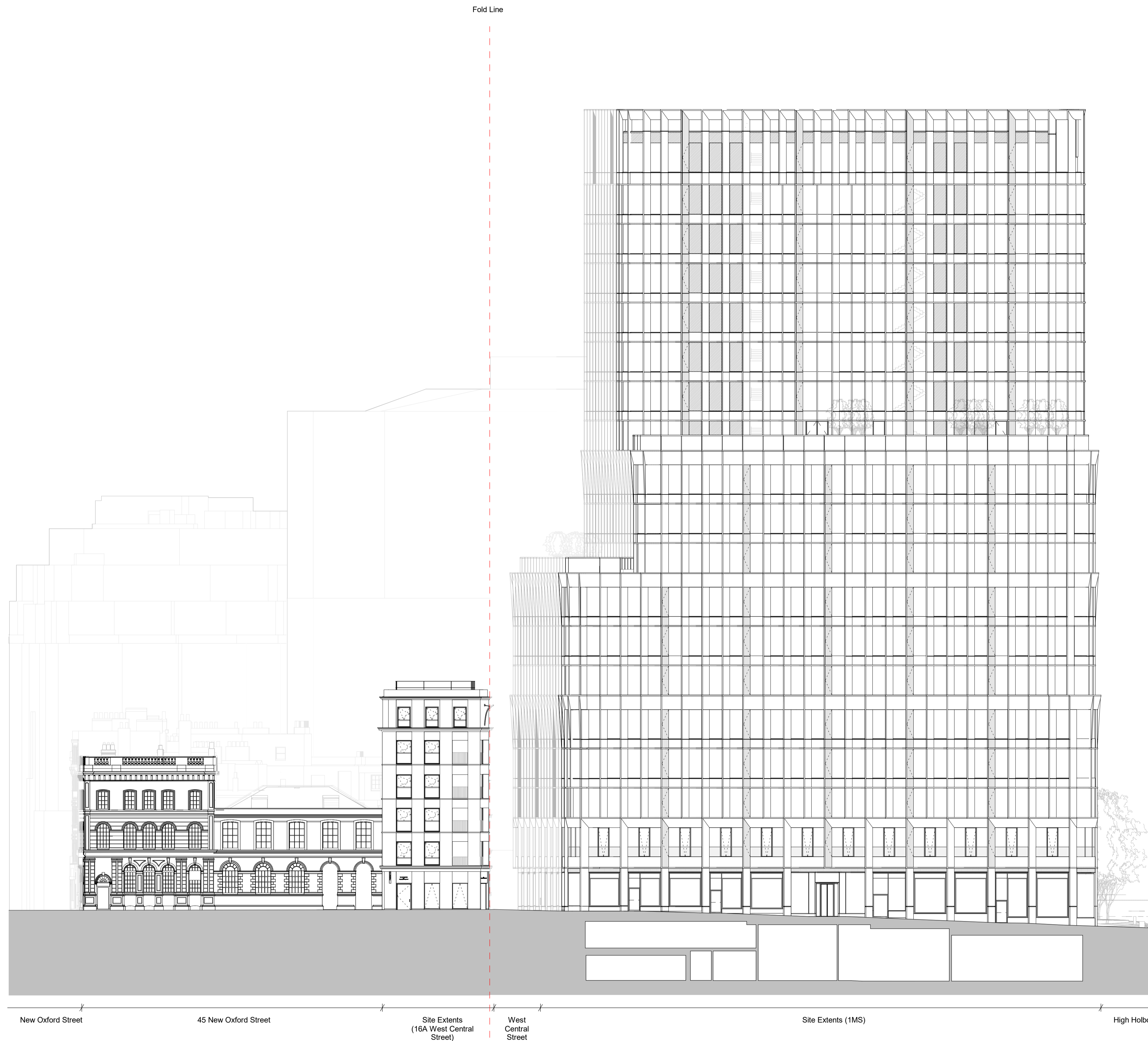
Proposed West Central Street Elevation - East
