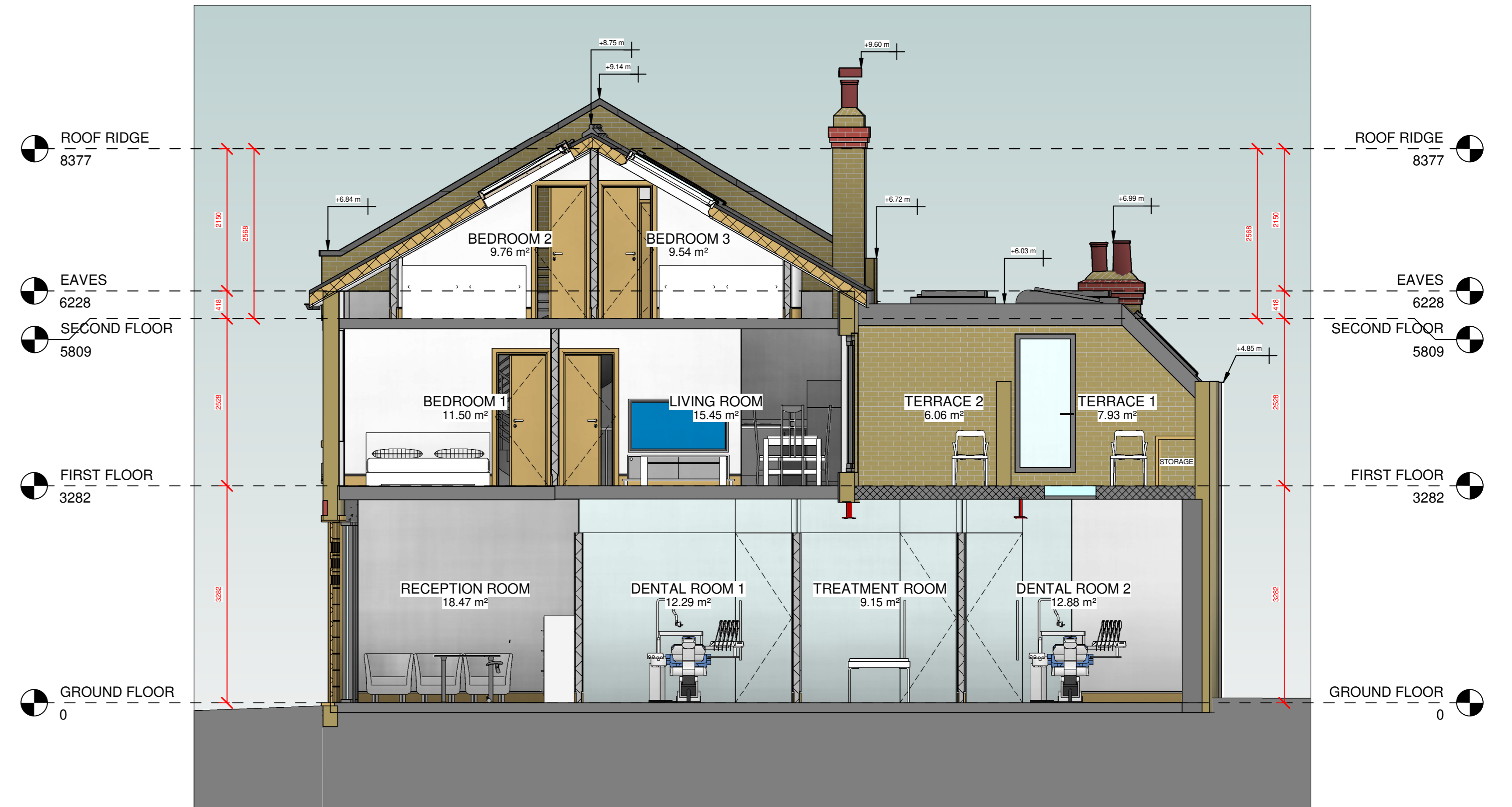
2 SECTION 2 1:50
