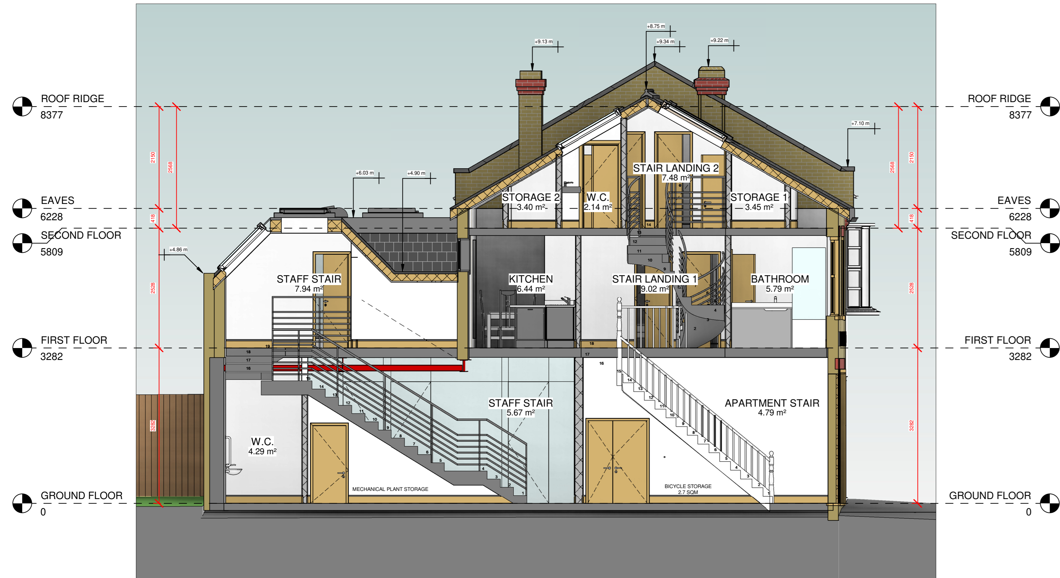
1 SECTION 1 1:50
