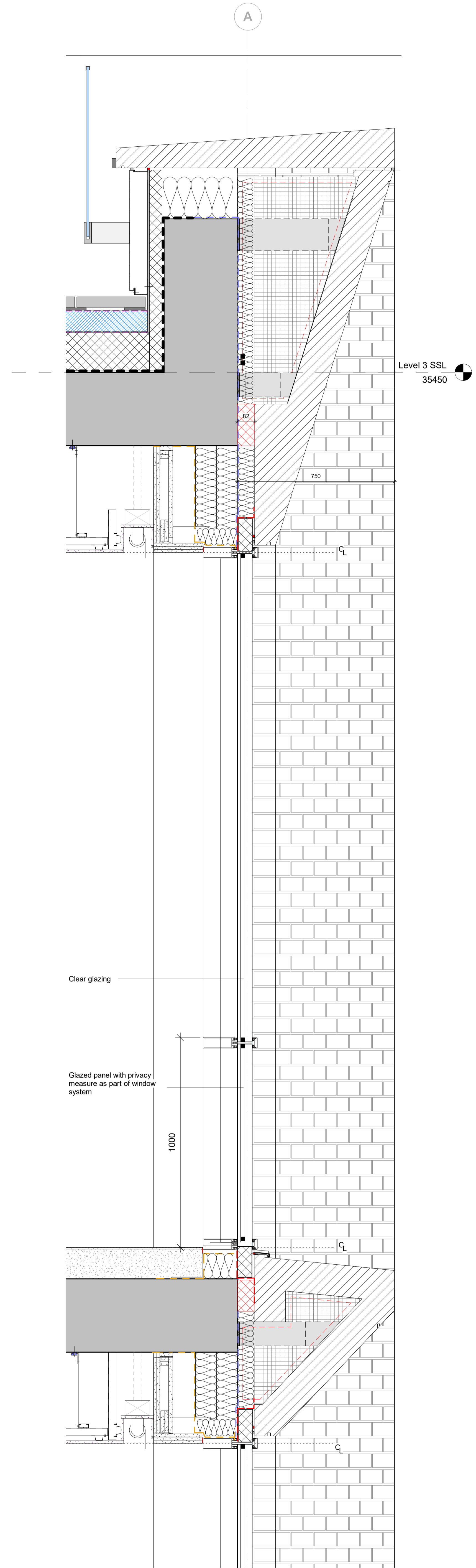
4 Section Detail (L02 / Gridlines 3-4 & A) 1 : 10
