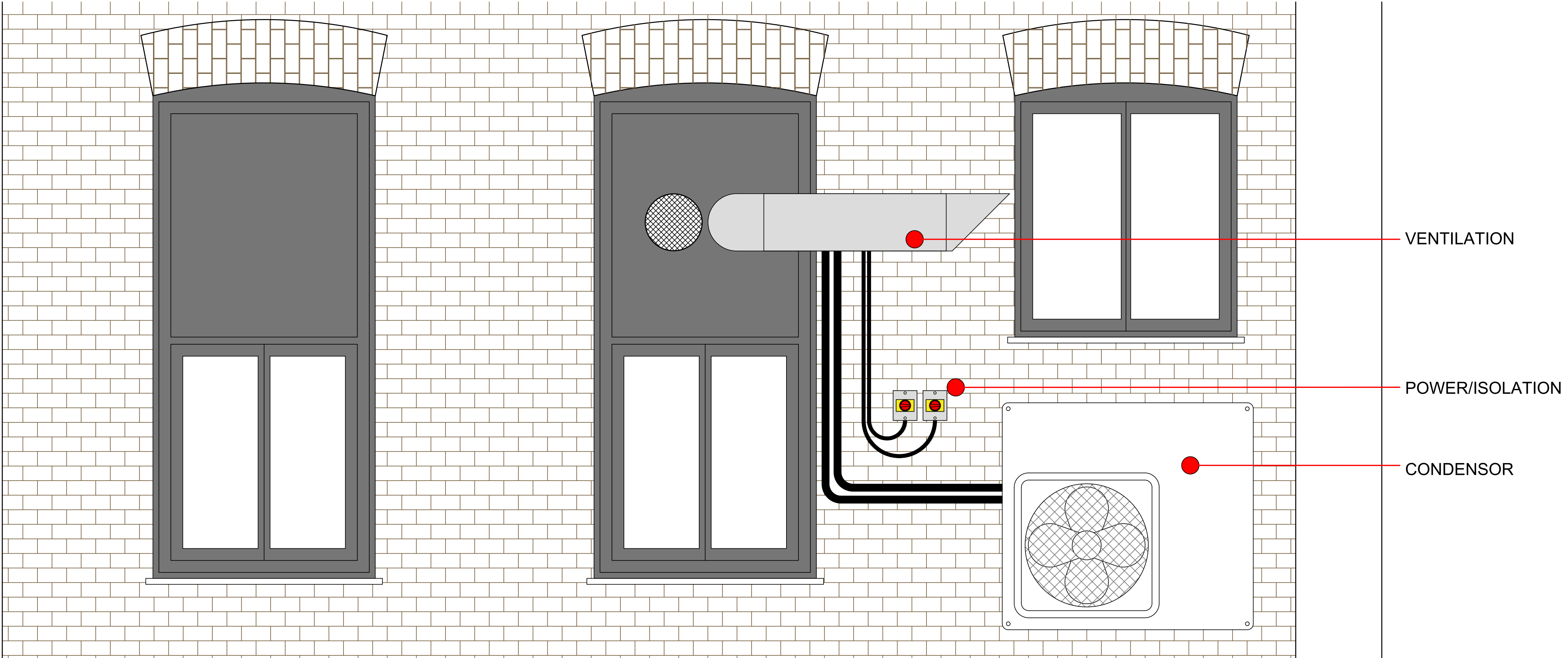
ELEVATION - OUTSIDE SPACE / TENANT ROOF AREA
