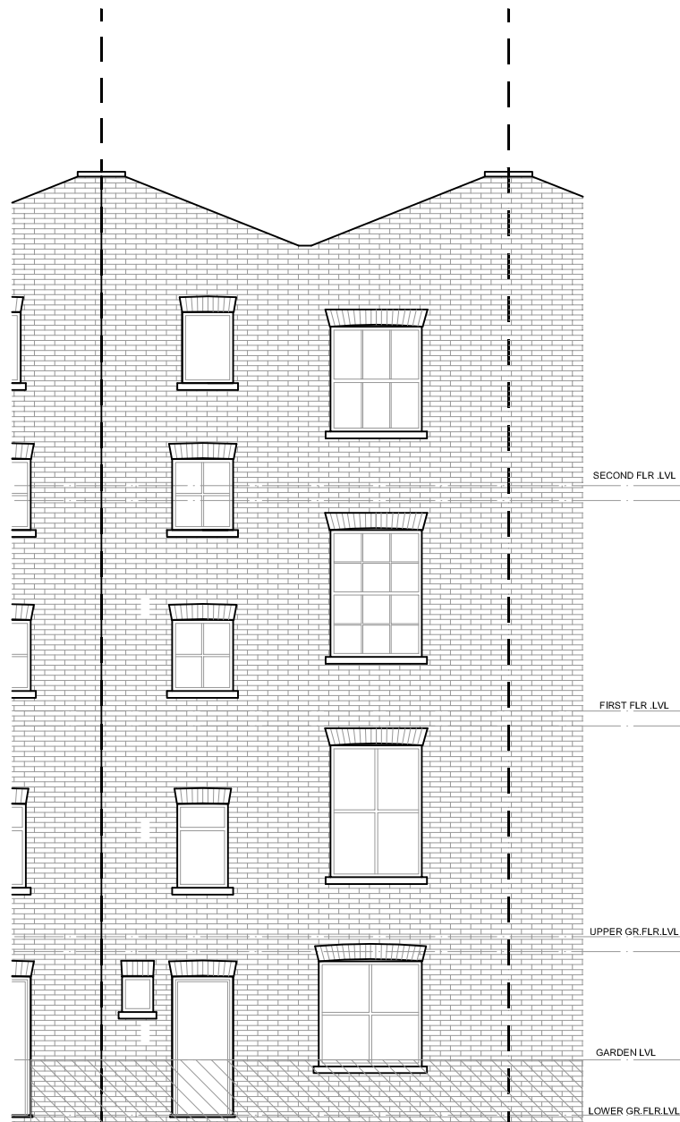
EXISTING/PROPOSED REAR ELEVATION
