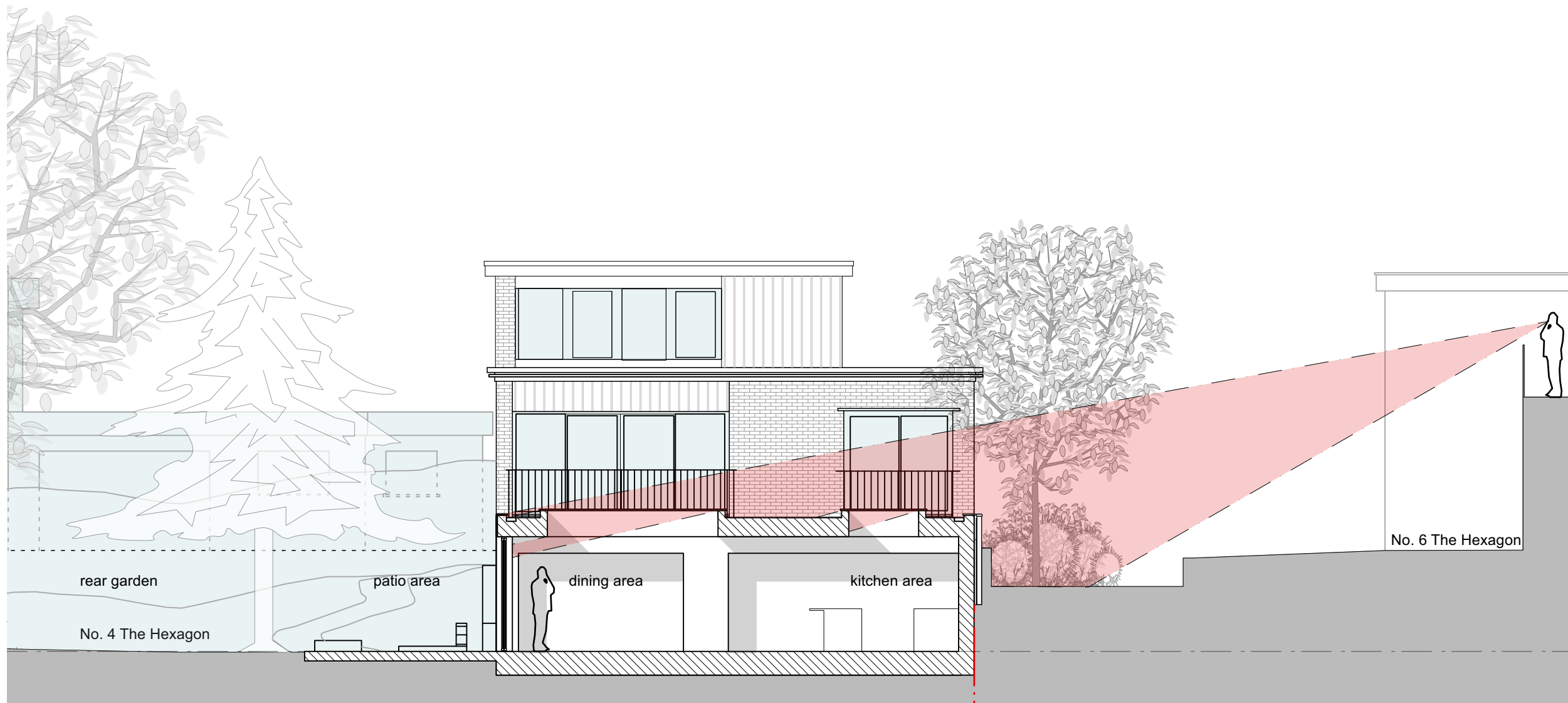
Section BB - View from property at number 6
