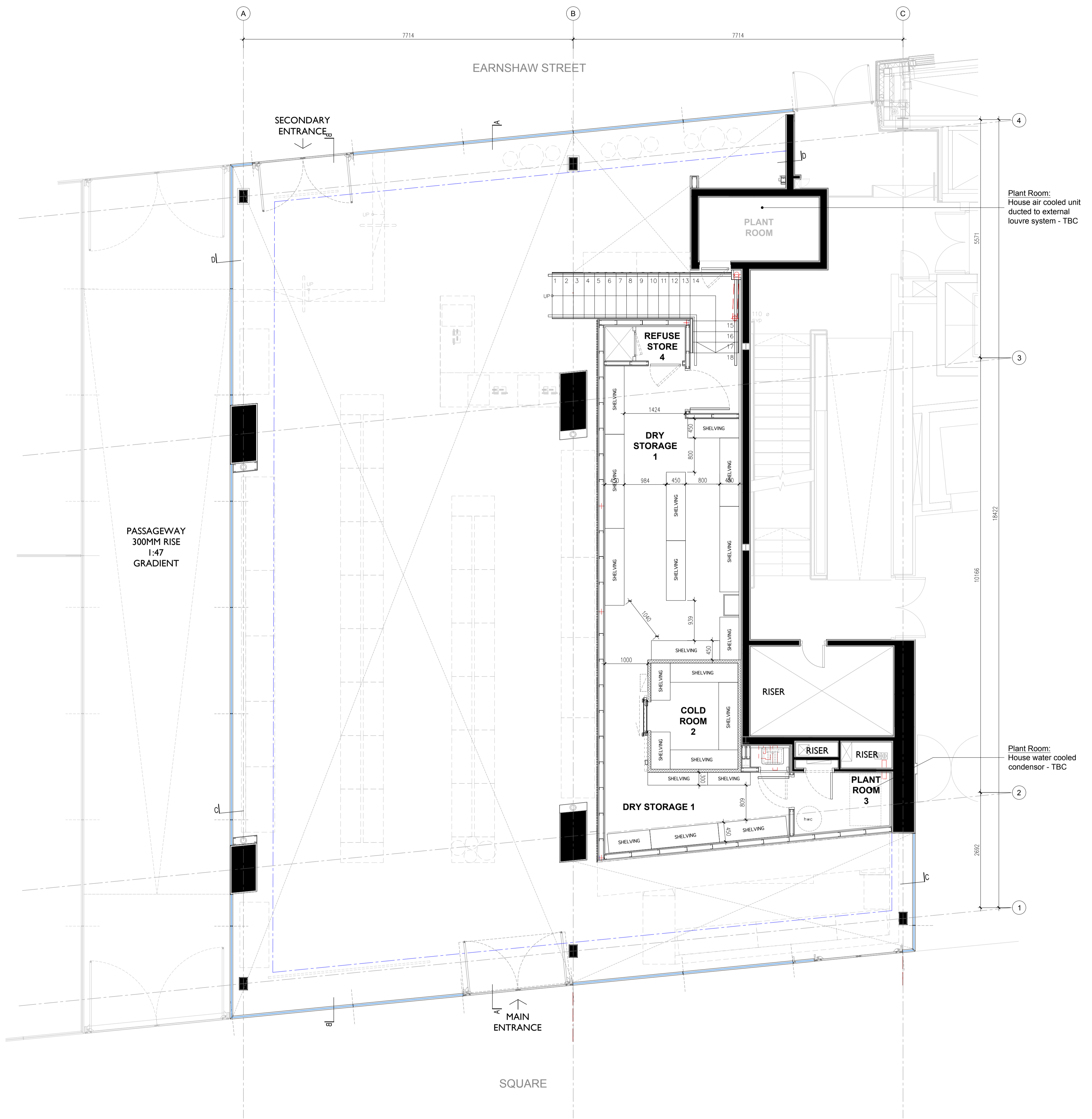
PROPOSED MEZZANINE FLOOR GENERAL ARRANGEMENT PLAN SCALE 1:50
