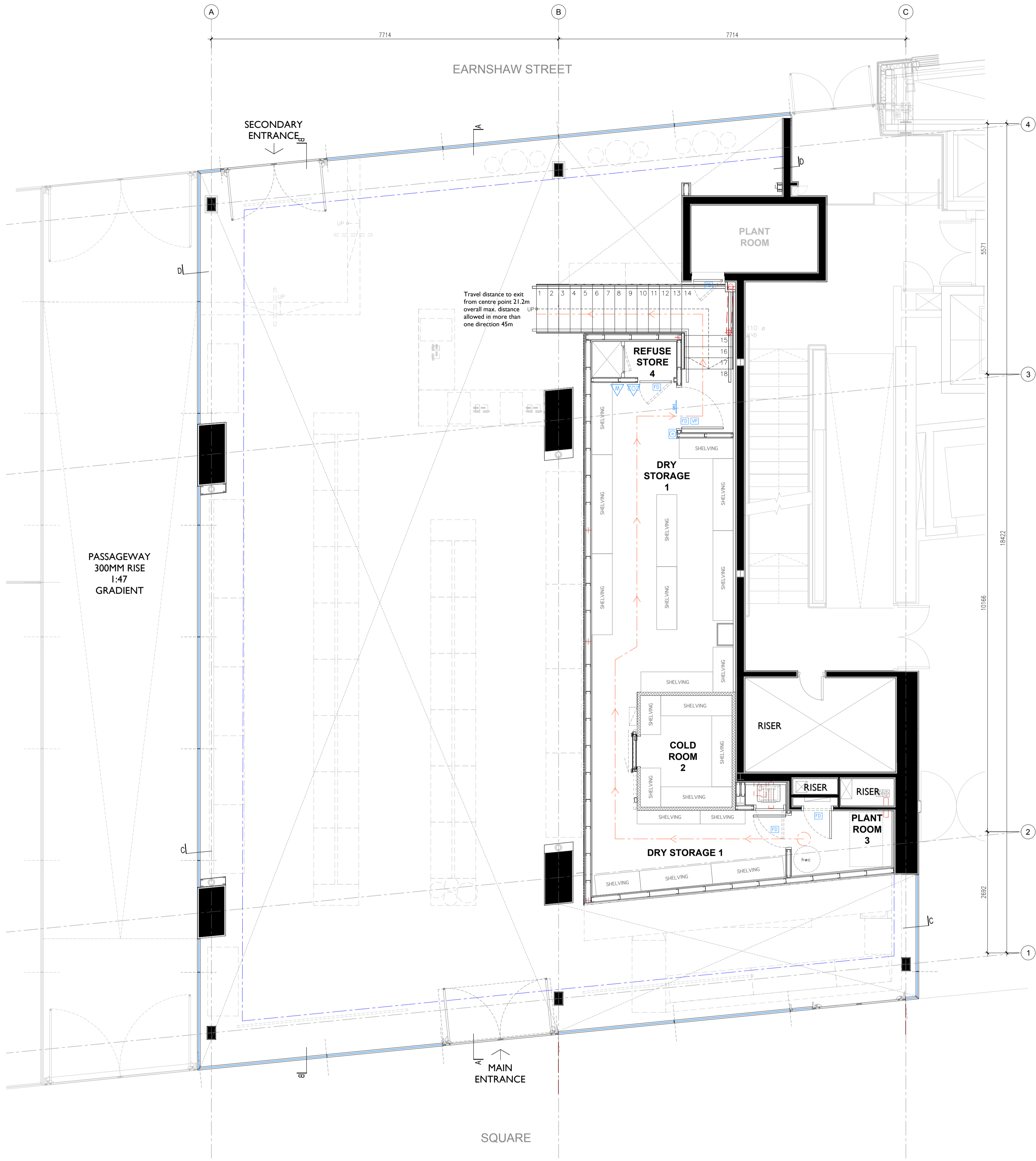
PROPOSED MEZZANINE FLOOR FIRE STRATEGY PLAN SCALE 1:50
