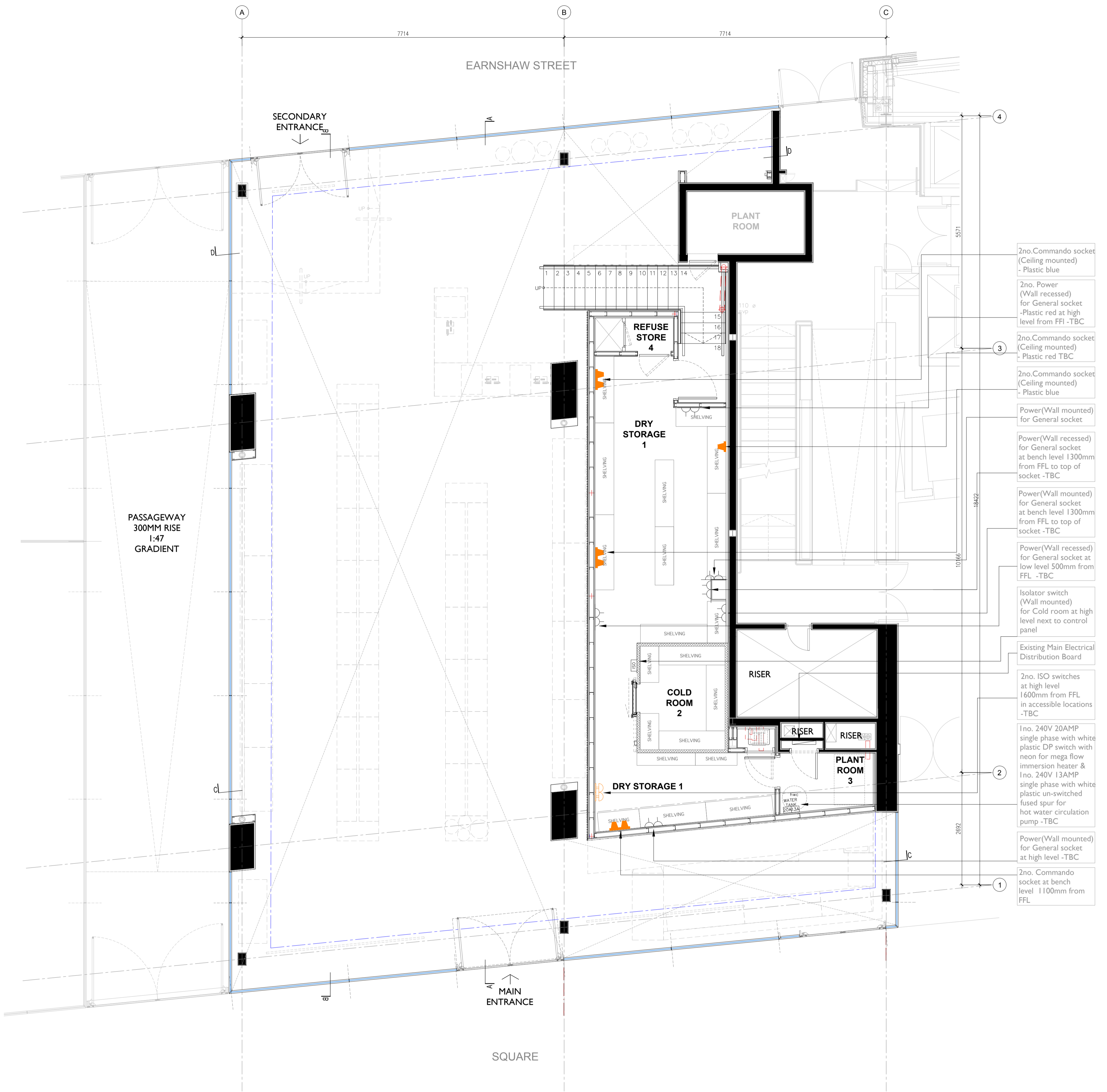
PROPOSED MEZZANINE FLOOR POWER & DATA LAYOUT SCALE 1:50
