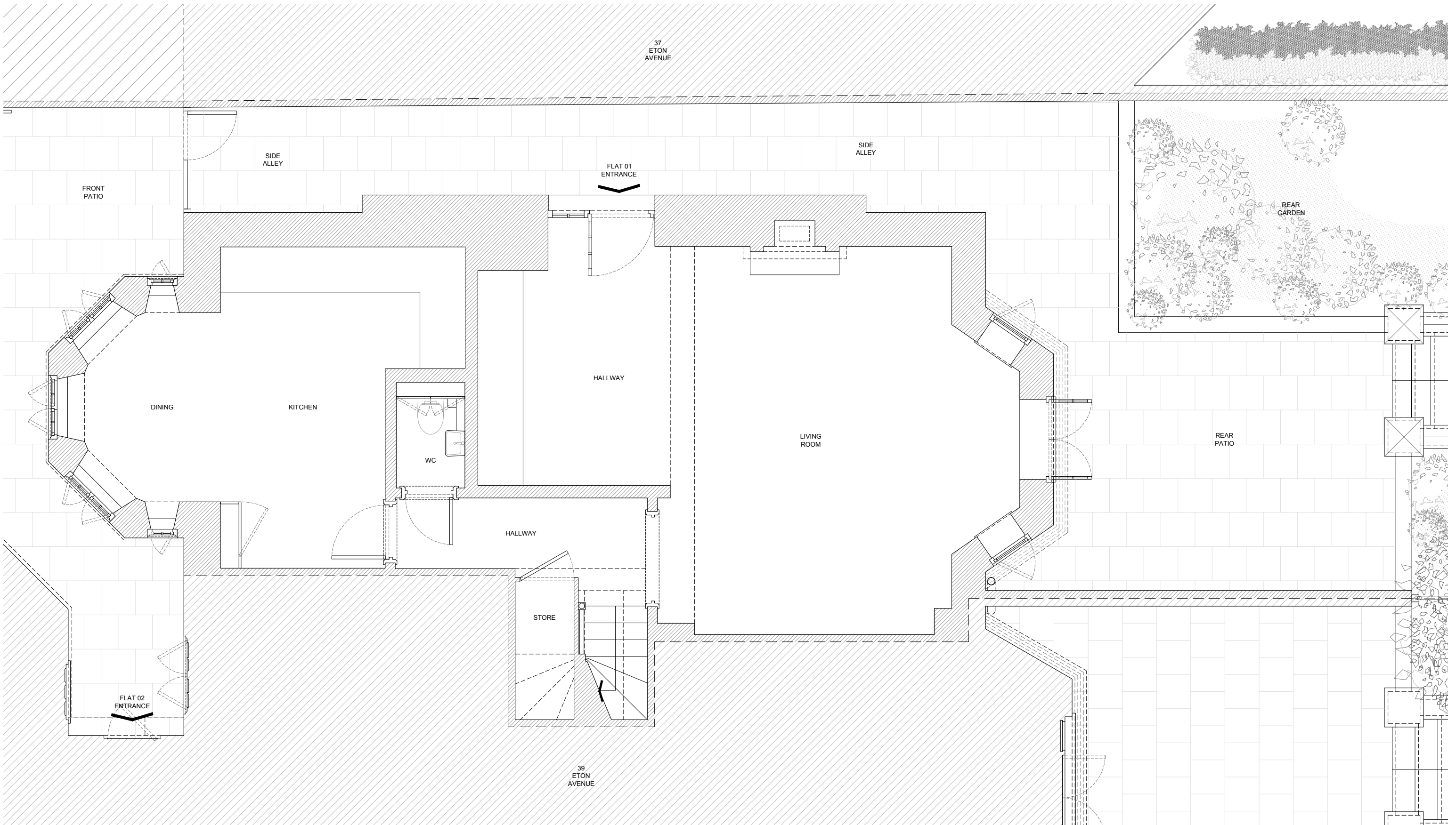
EXISTING LOWER GROUND FLOOR PLAN 1:50 / A3
