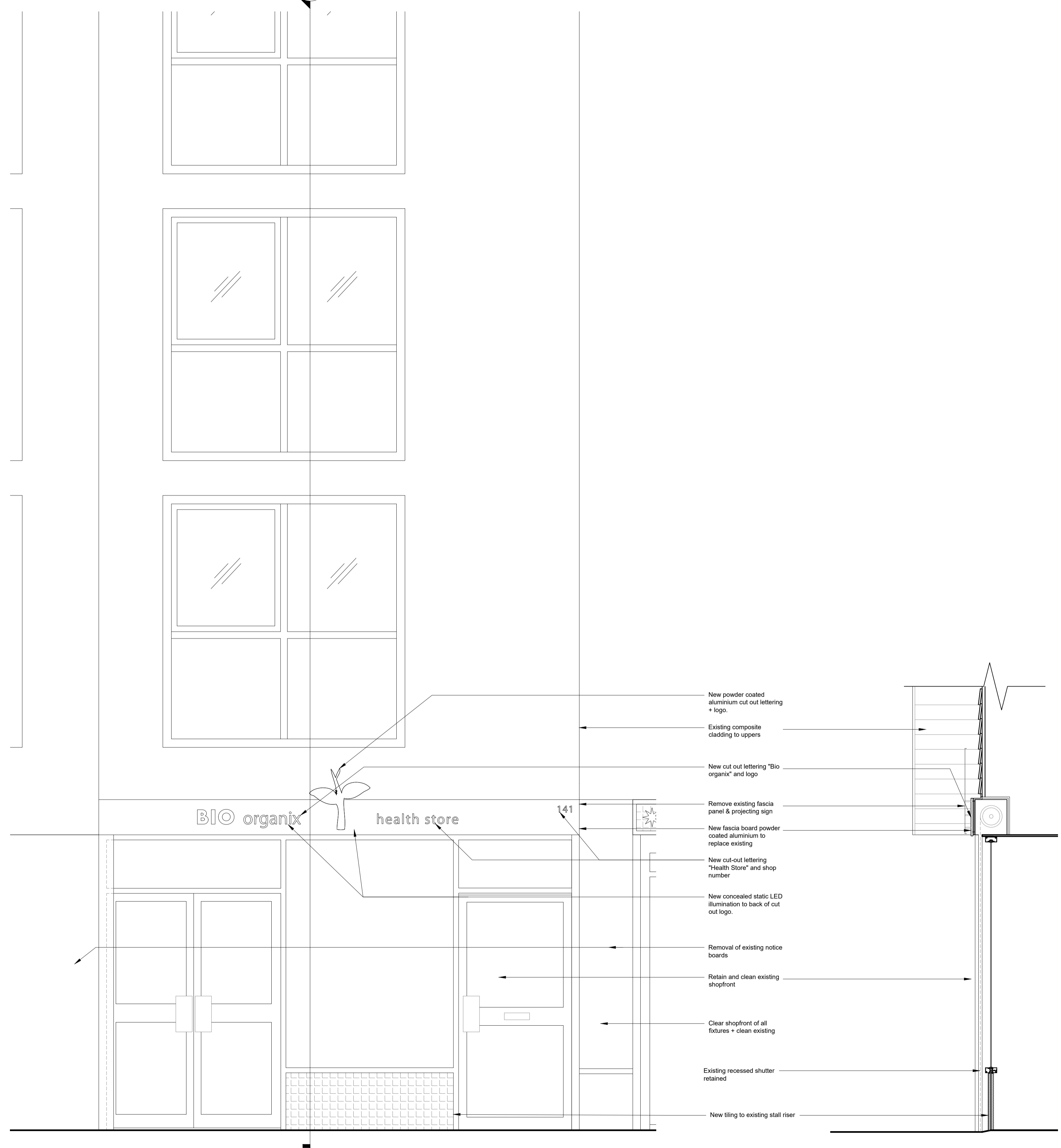
01 Proposed Elevation
